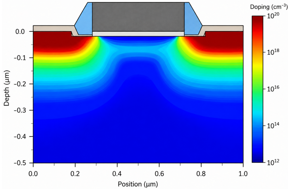
Figure 2: Typical TCAD simulation of a MOS transistor showing the spatial distribution of doping concentration.
