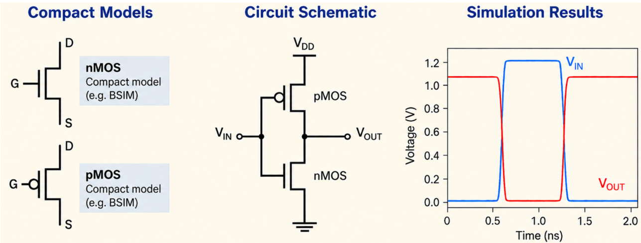
Figure 3: Functional circuit behavior is predicted by combining compact device models in circuit-level simulation.
