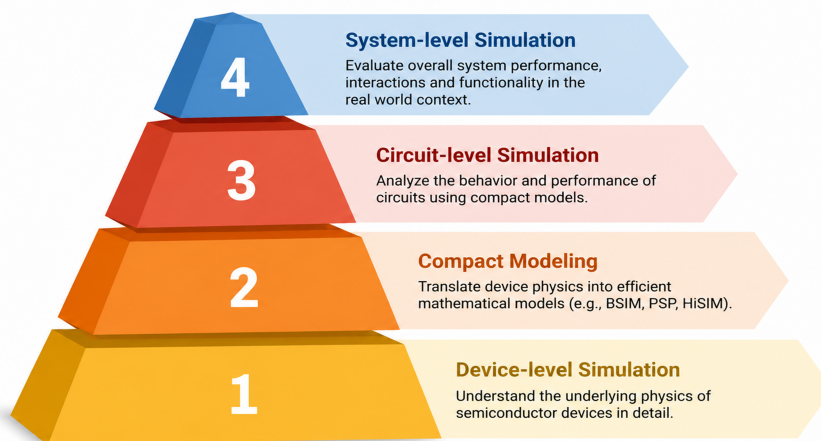
Figure 1: The hierarchy of semiconductor models: from devices to systems.
