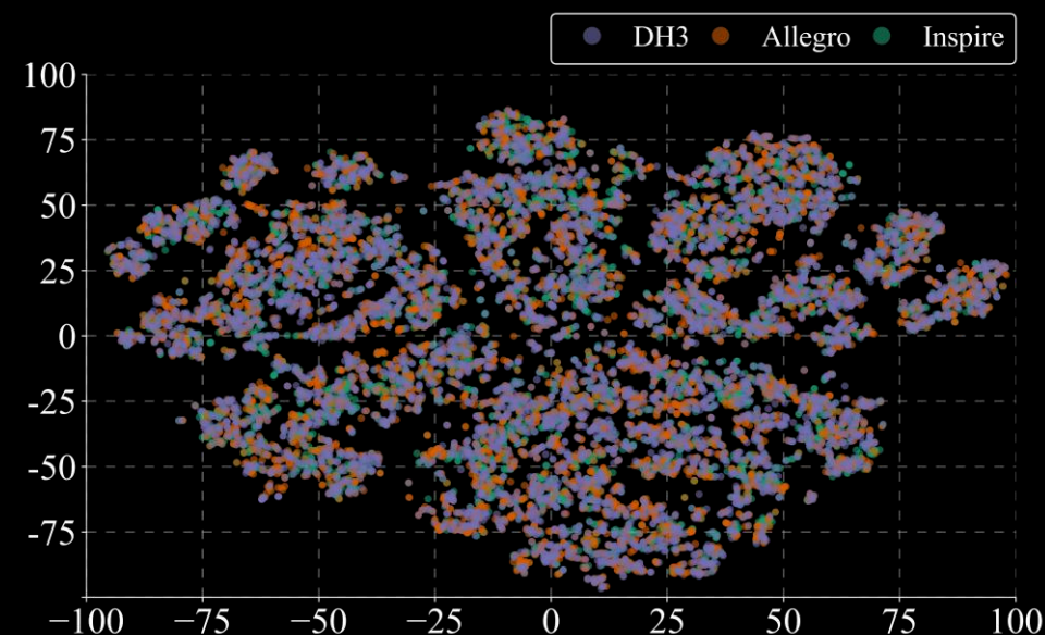
(c) Hand-agnostic HOI Space
