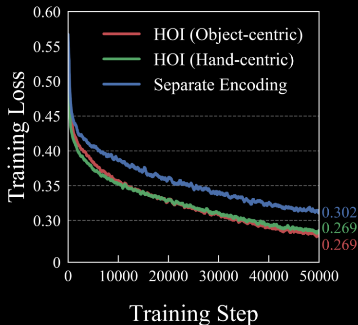
(a) Training Convergence
