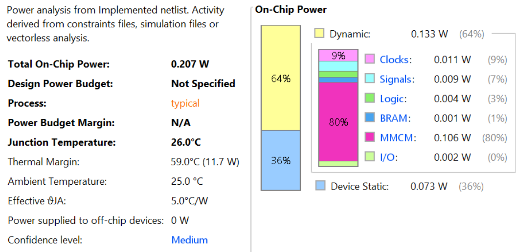
Gambar L.19. Power summary report - total on-chip power consumption, breakdown per resource (MMCM, Block RAM, Slice Logic), dan power supply margins
