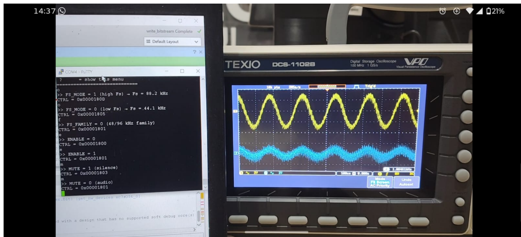
Gambar L.10. Hasil capture osiloskop: Mute=0 (unmuted) - audio normal dioutput
