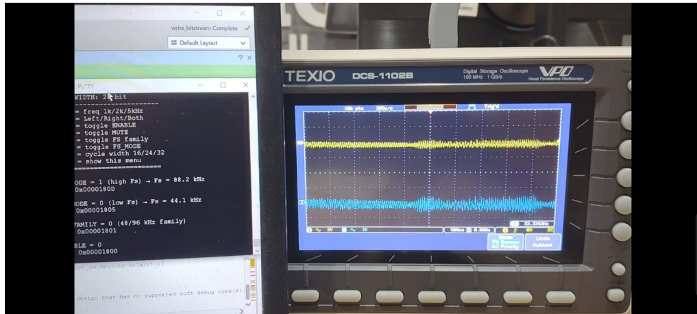
Gambar L.8. Hasil capture osiloskop: Enable=0 (disabled) - I2S transmitter off
