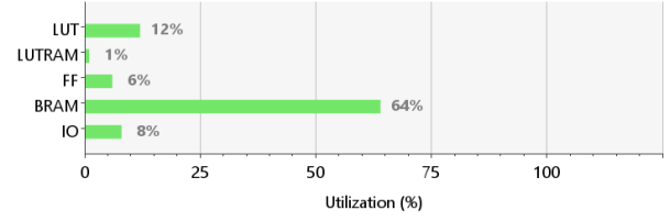
Fig. 2. Resource utilization summary of the implemented SoC and I2S transmitter.
