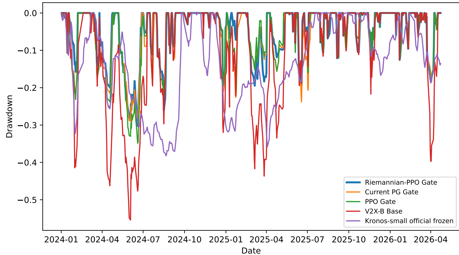
Main Drawdown Comparison with Riemannian-PPO Final Controller
