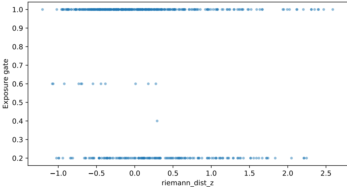
SPD-Riemannian market-state distance vs exposure gate
