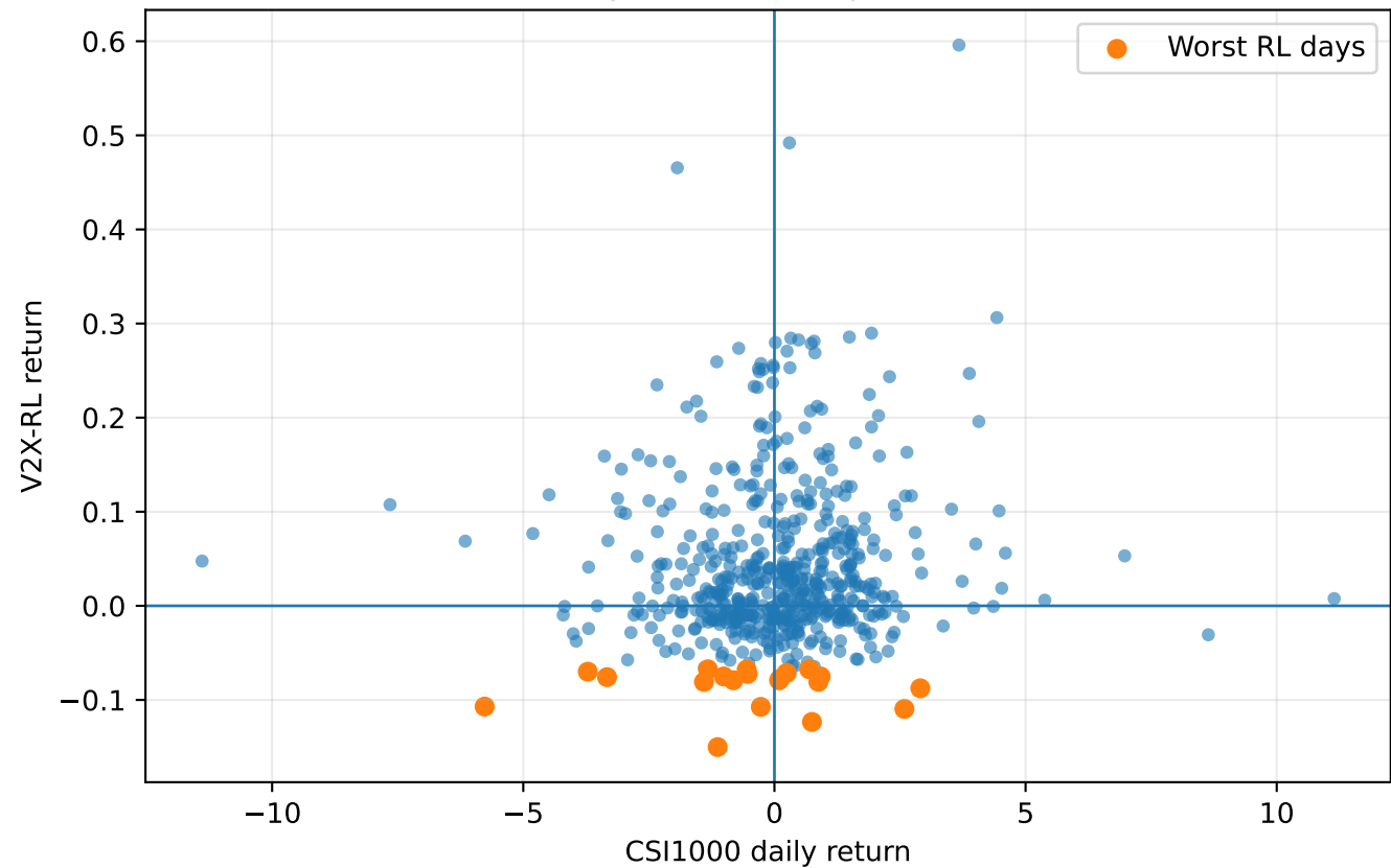
Failure Days vs Small-cap Market State
