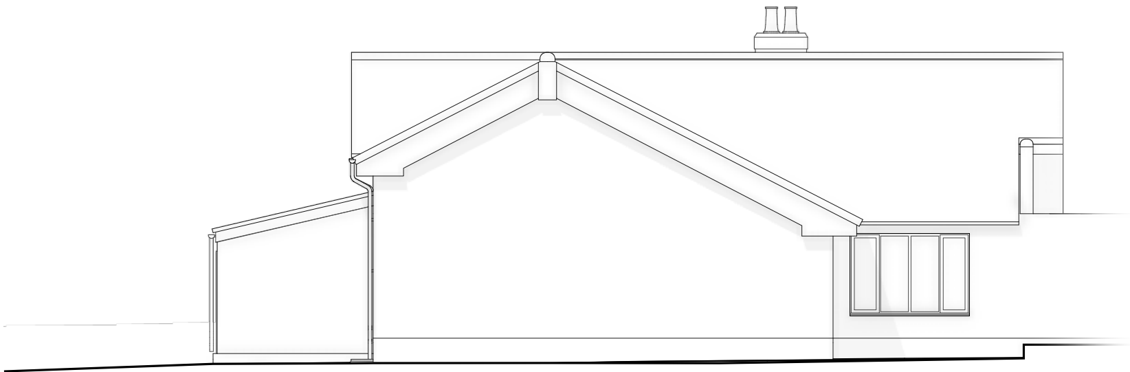
Existing West Elevation – Rear Of Dwelling
