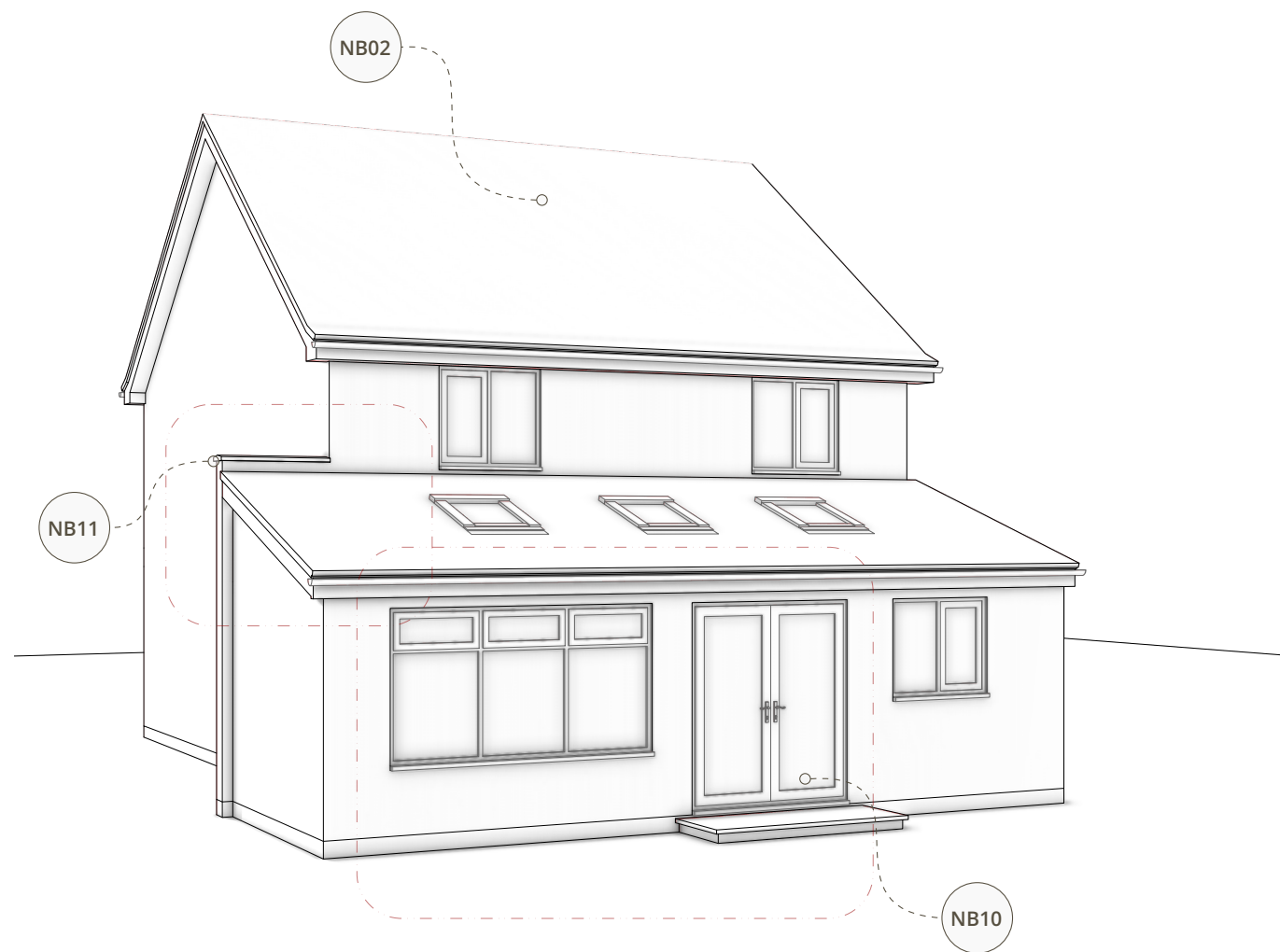
EXISTING SOUTHERN FACING FACADE
