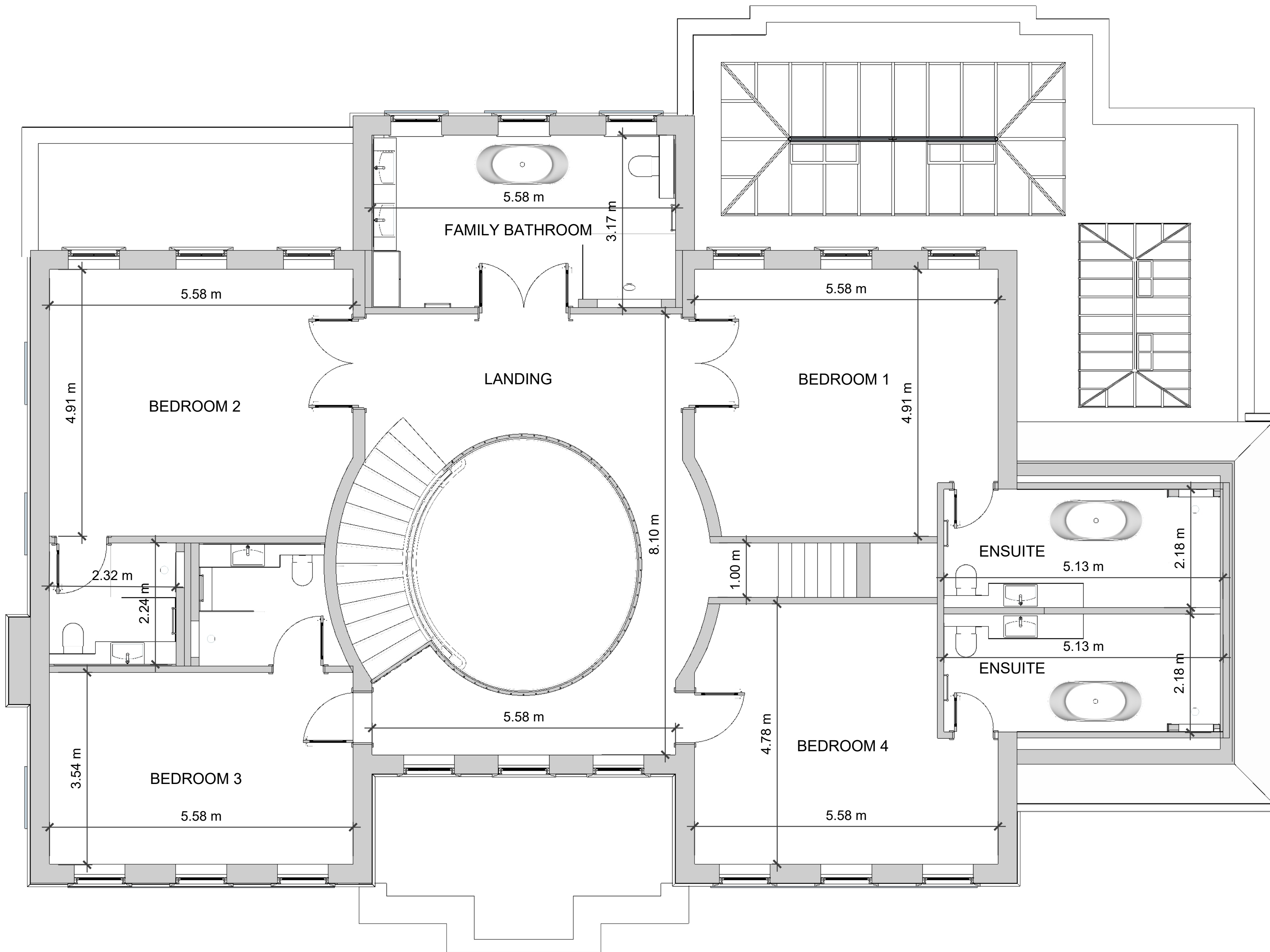
P2 Proposed First Floor Plan Scale: 1:50 @ A1
