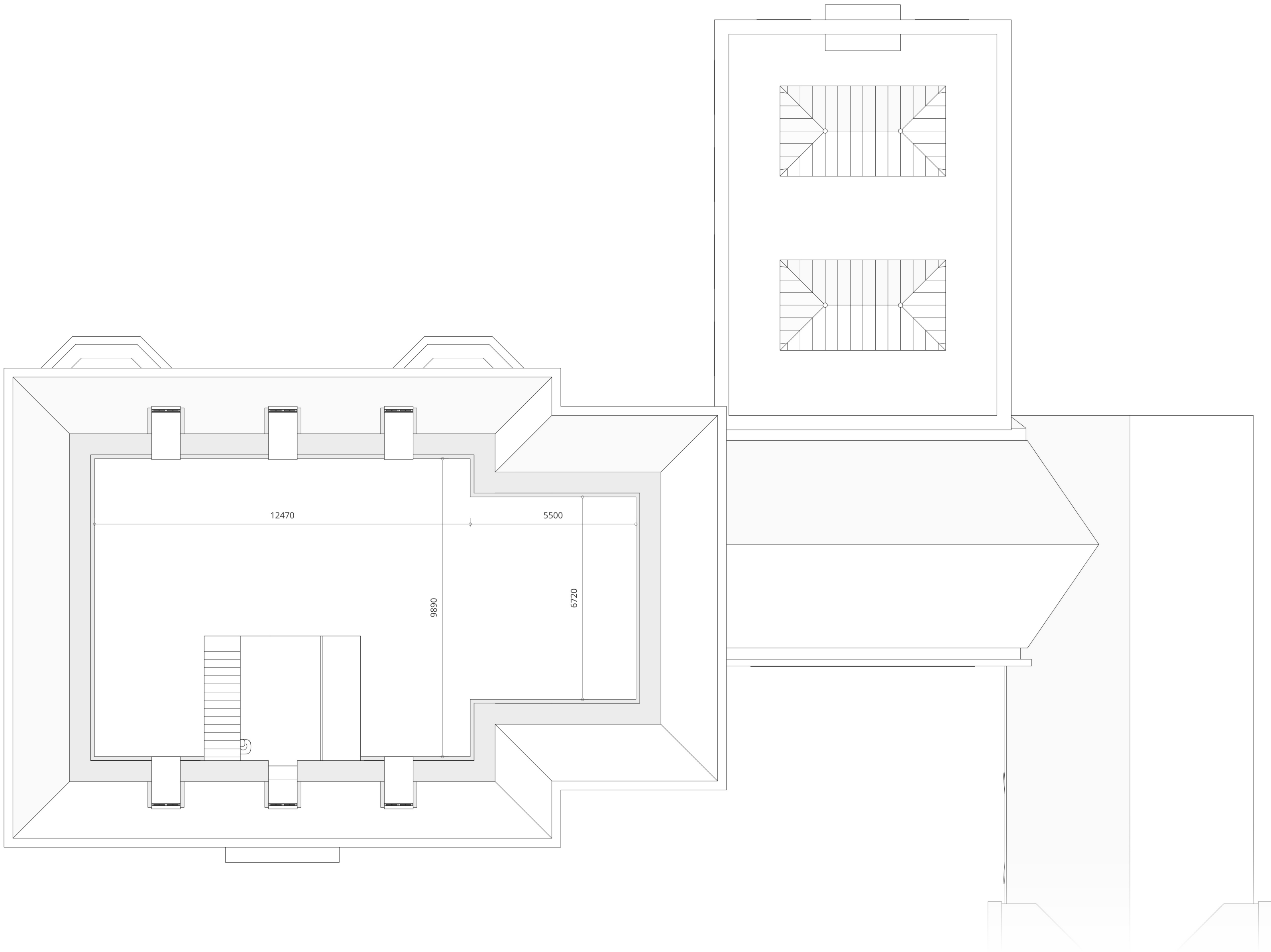
Second Floor | General Arrangement Plan – Main Residence
