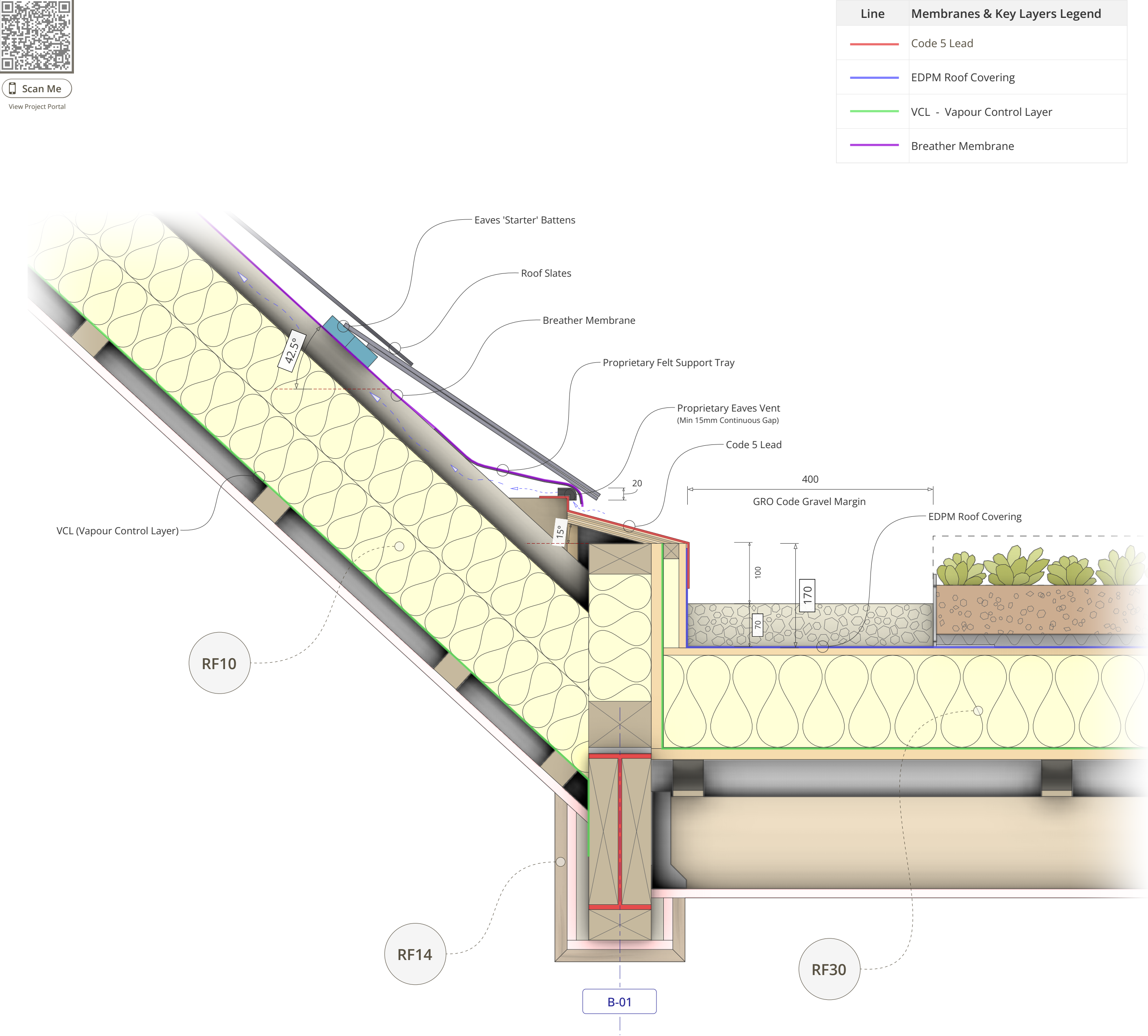
RF12 - Pitched Roof To Green Roof Abutment Detail
