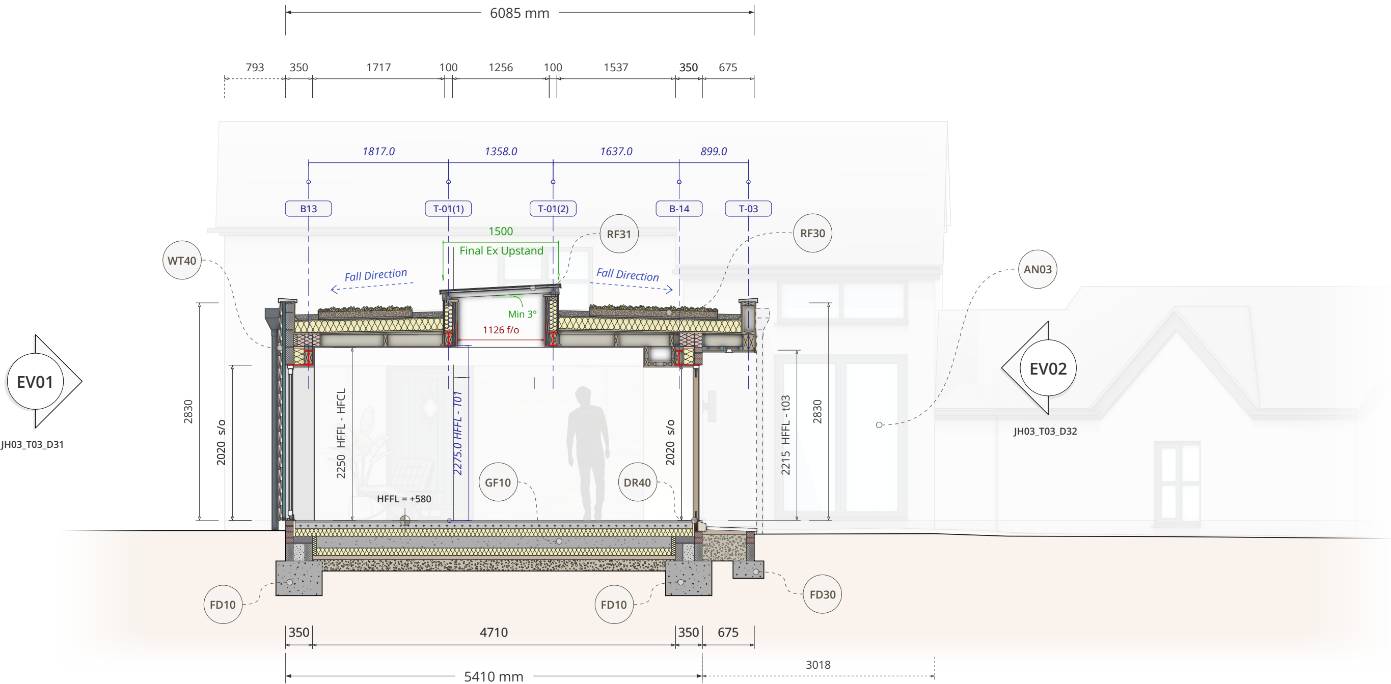
Technical Cross Section : C - C
