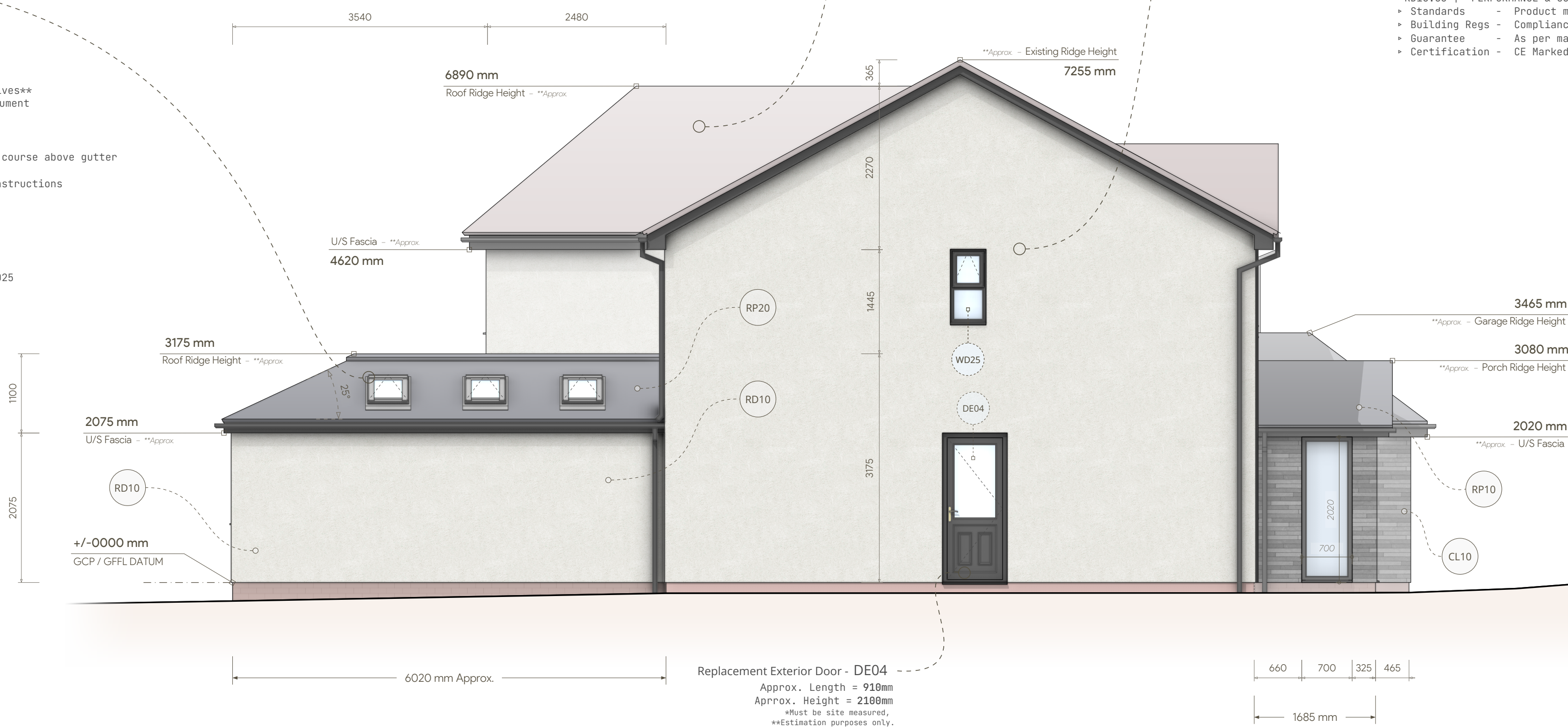
PE04 | West Elevation
