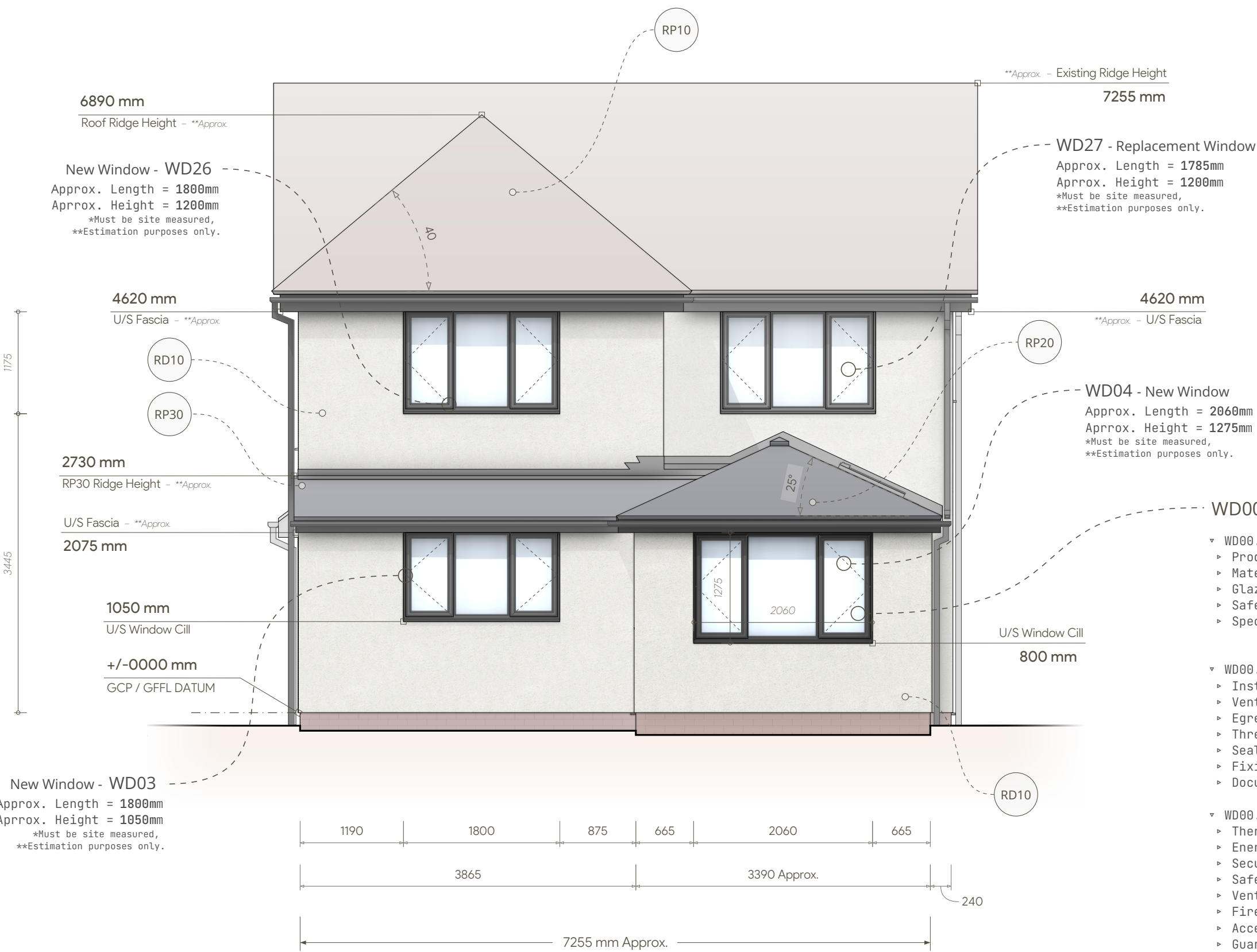
PE03 | South Elevation
