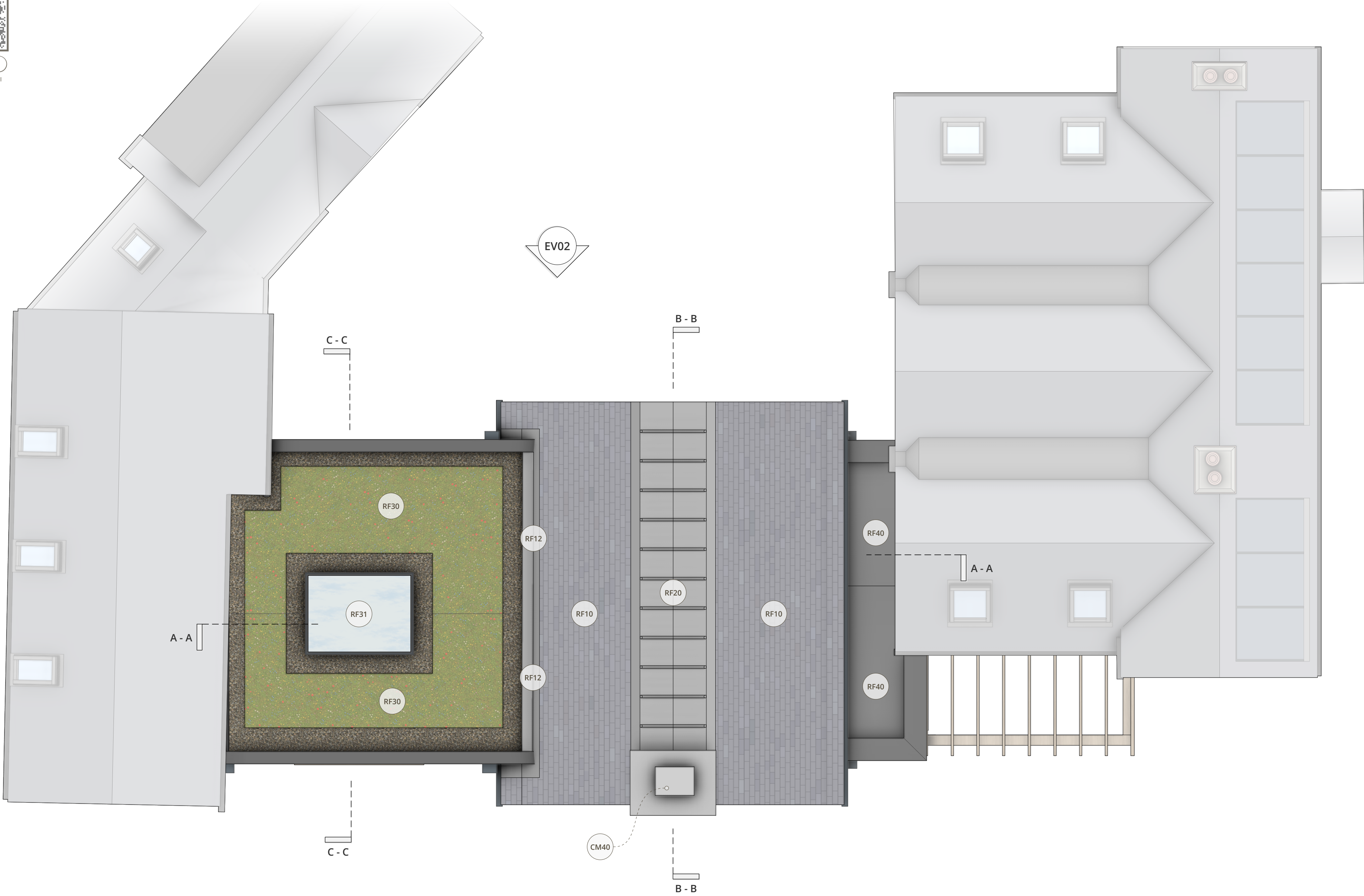
Proposed Extension Roof Plan
