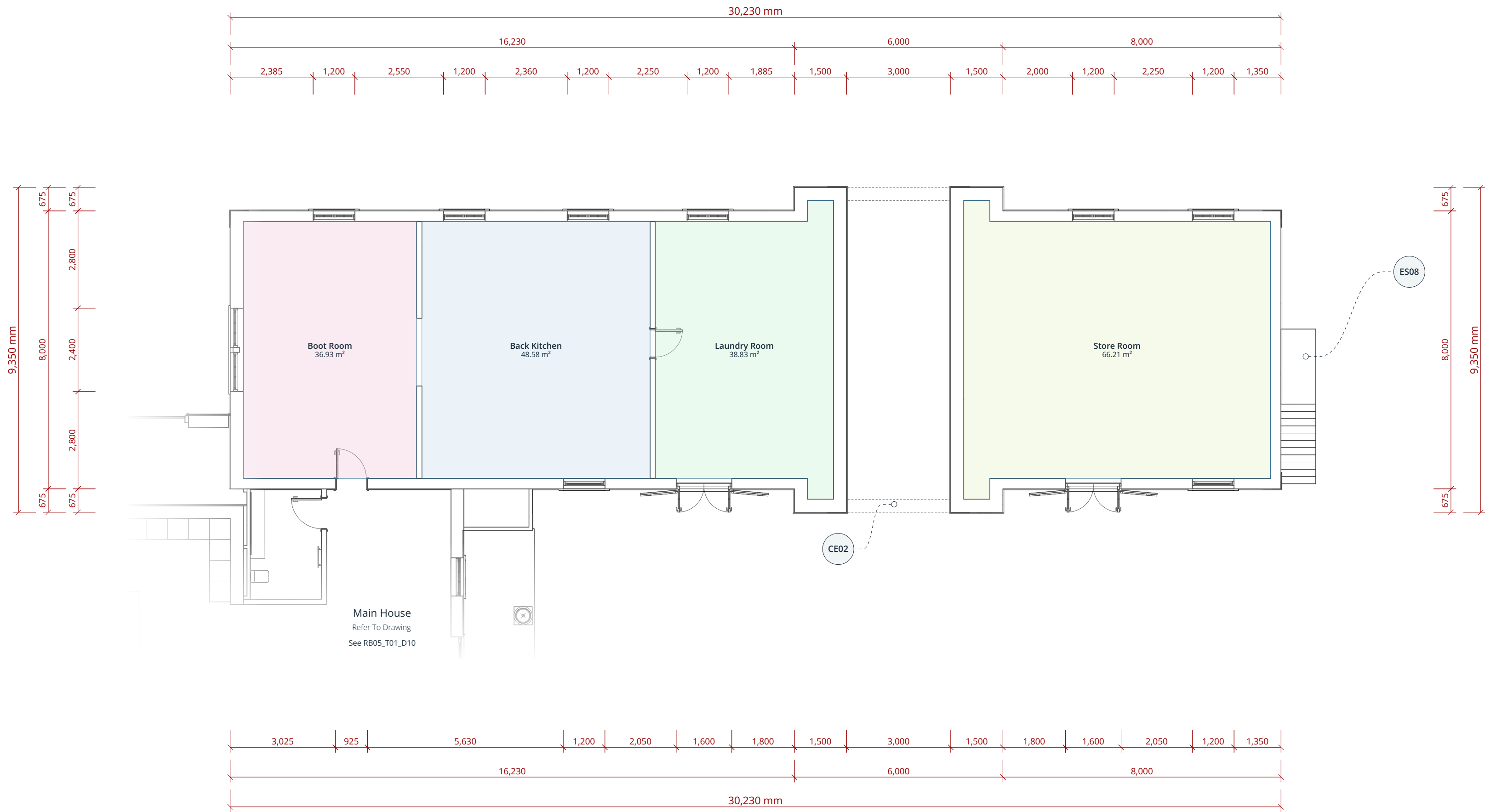
PROPOSED GROUND FLOOR PLAN - COACH HOUSE
