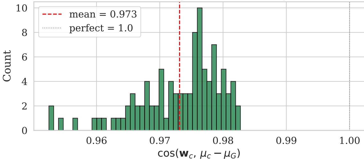
NC3: Classifier weight / class mean alignment
