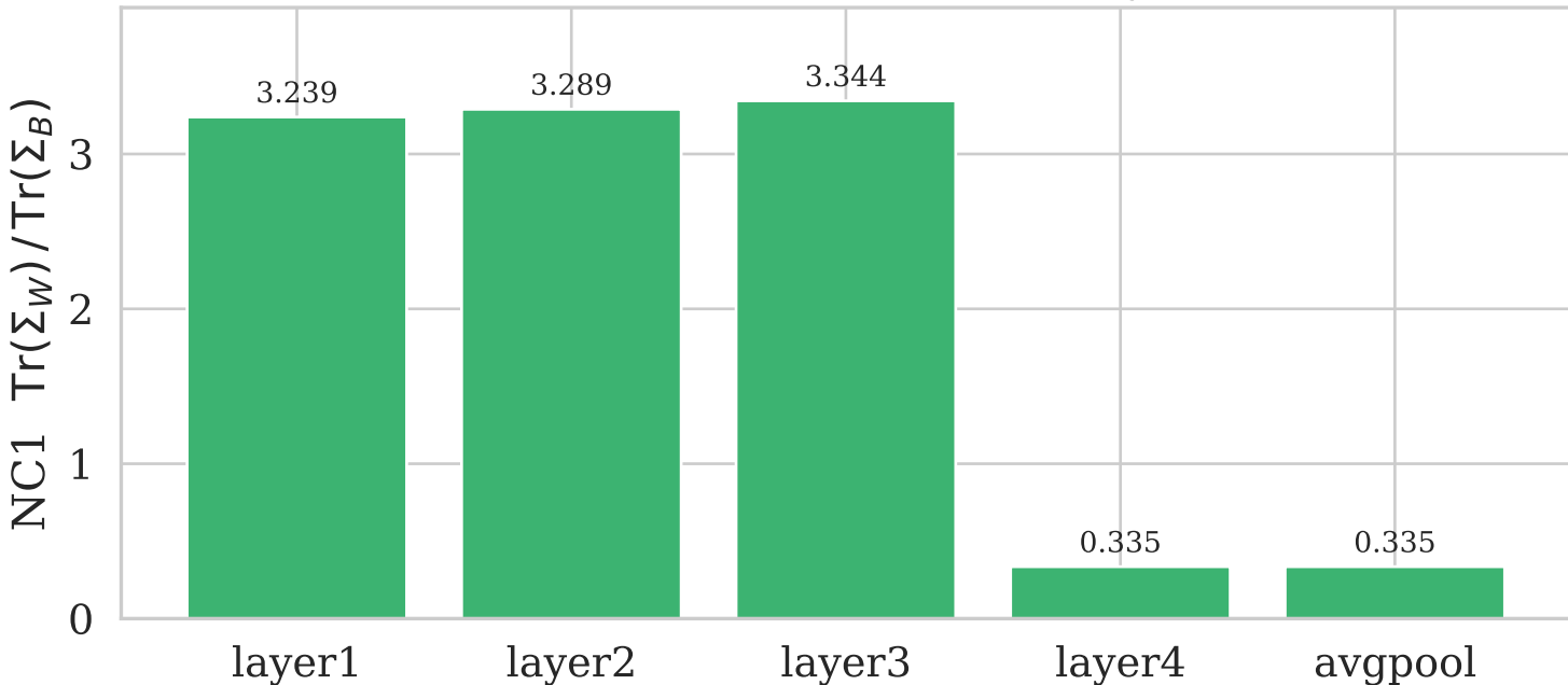
Neural Collapse (NC1) across ResNet-18 layers — final model
