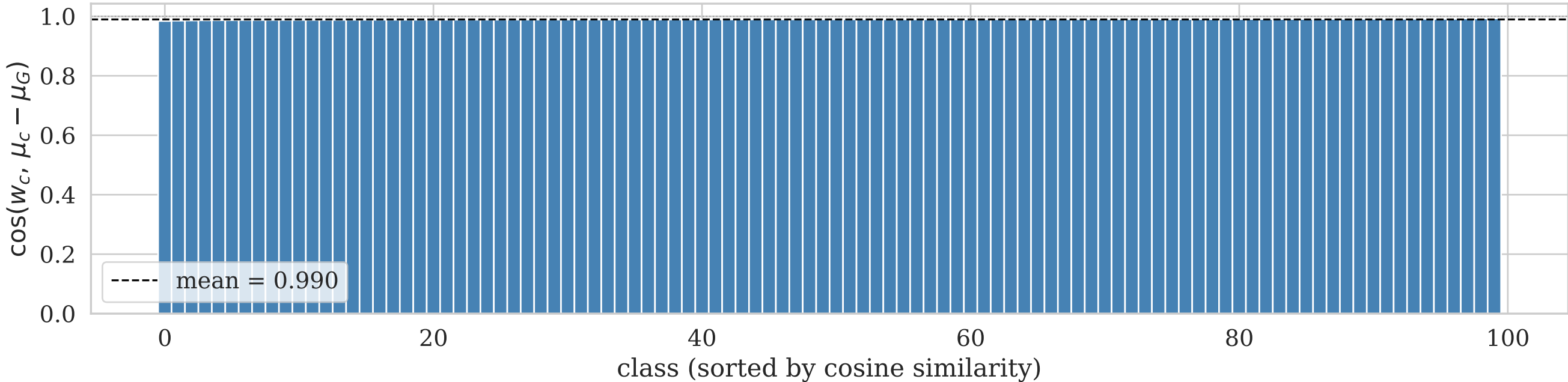
Per-class cosine similarity: classifier weight vs centered class mean (NC3)
