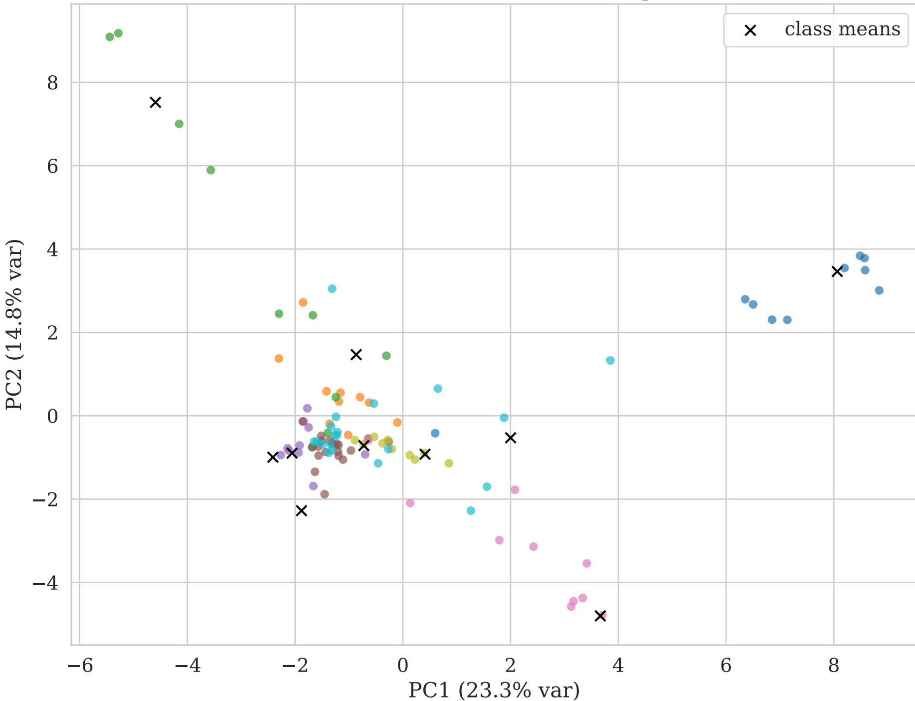
PCA 2D — 10 CIFAR-100 classes (10 pts each)
