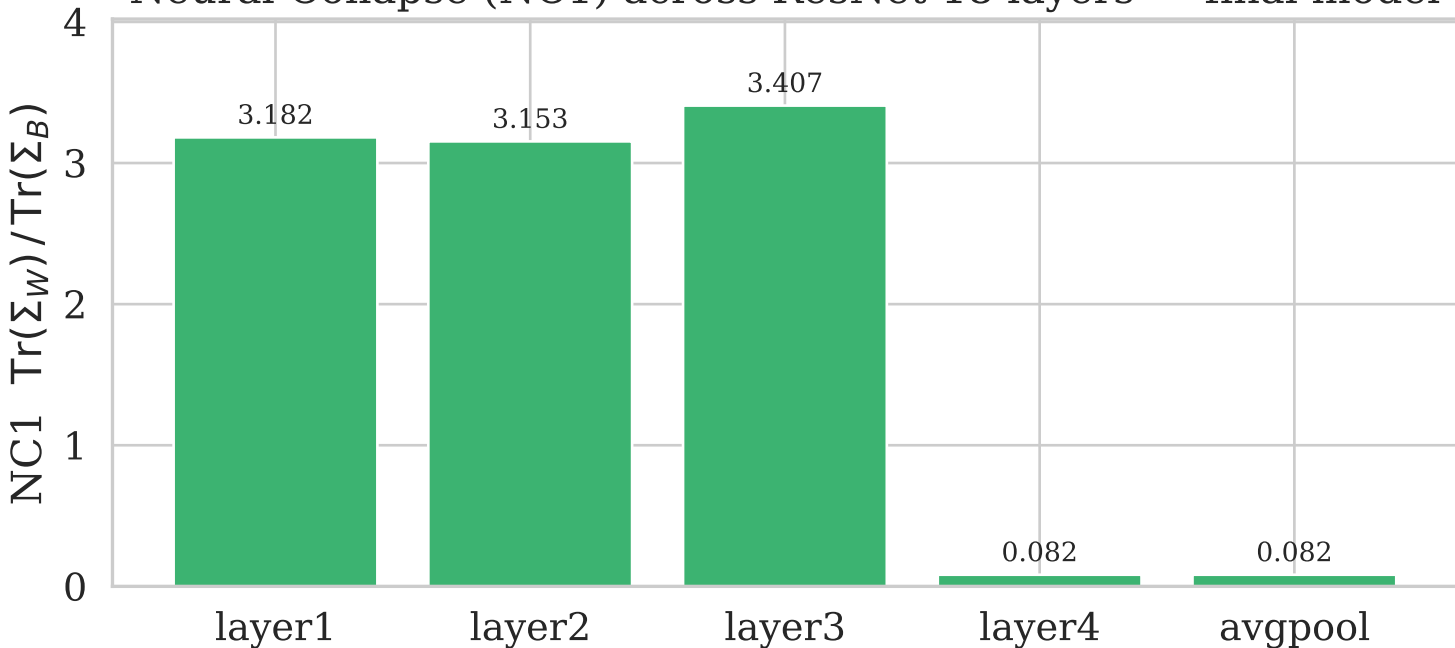
Neural Collapse (NC1) across ResNet-18 layers — final model
