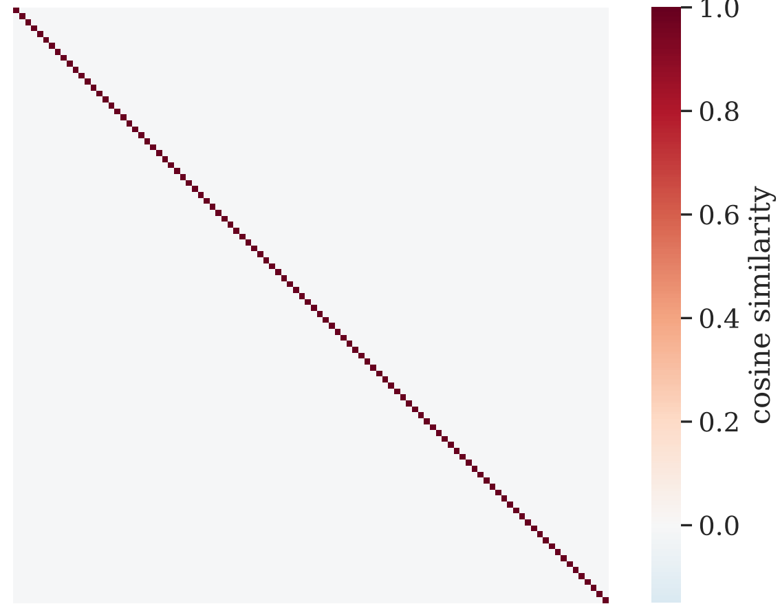
Ideal ETF Gram matrix
