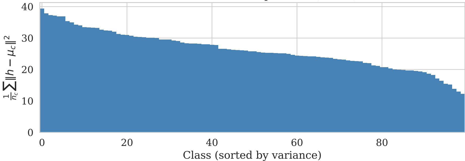
Within-class variance per class (sorted)
