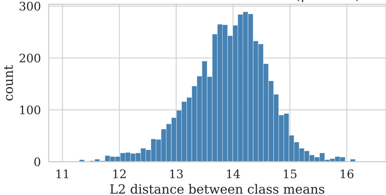
Distribution of inter-class mean distances ( \mu=13.93 , \sigma=0.69 )
