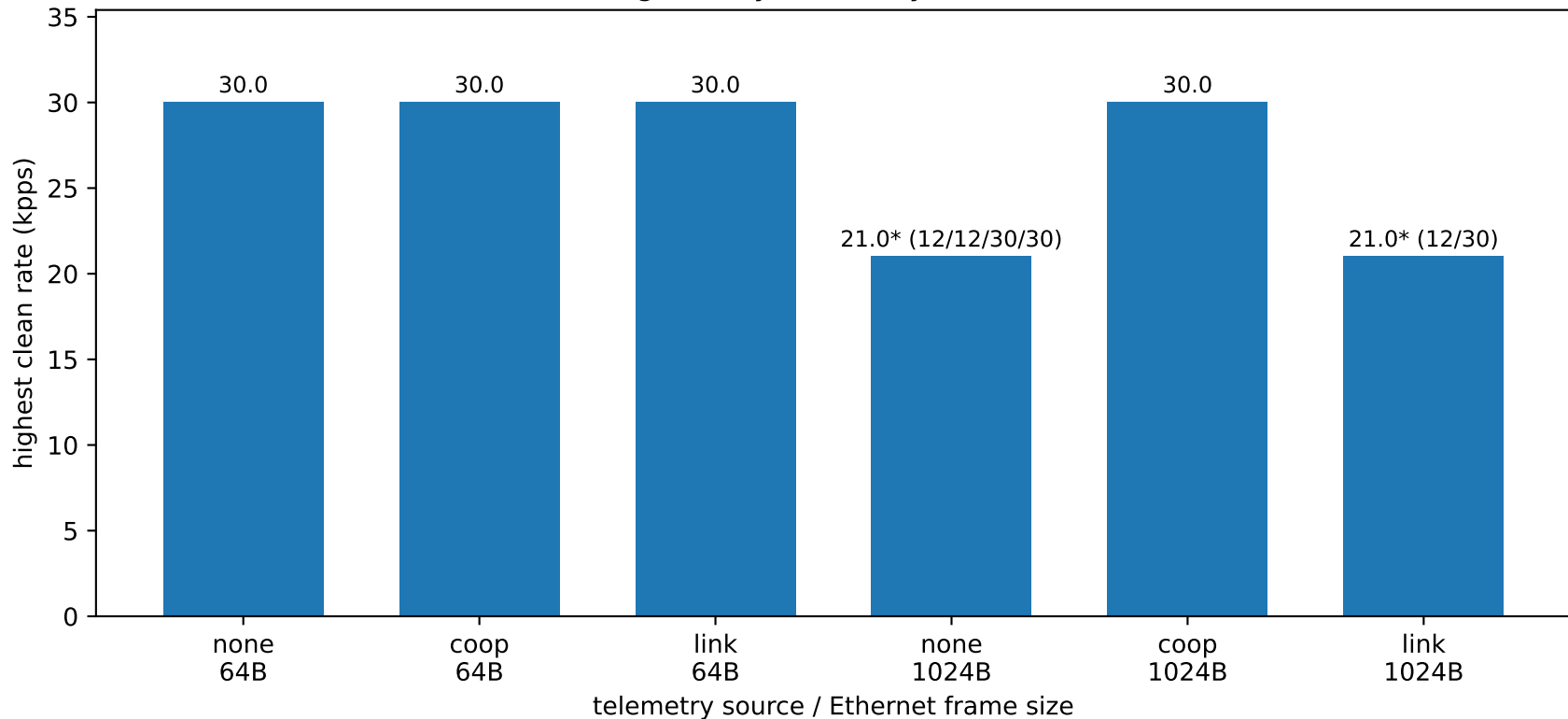
Clean forwarding rate by telemetry source and frame size
