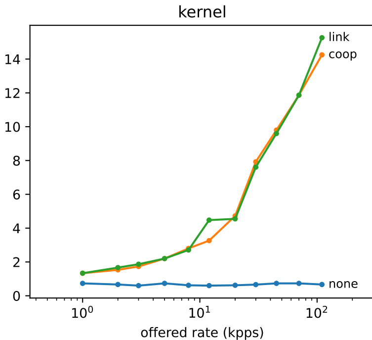
CPU by telemetry source and offered rate (1024 B frames)
