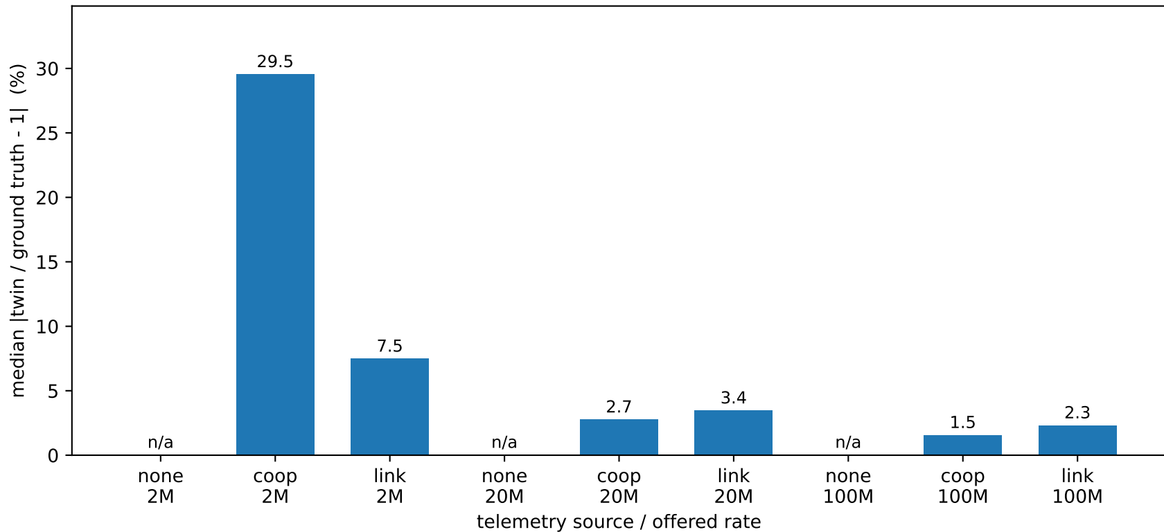
Twin bandwidth error against /proc/net/dev, by telemetry source
