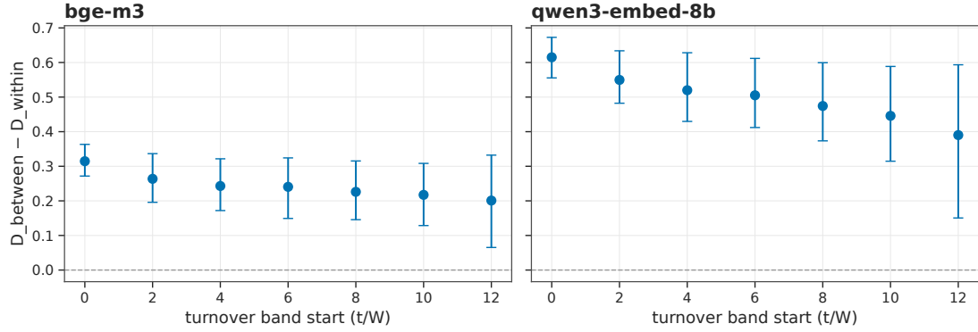
Figure 4: Between-seed last-band gap versus turnover in bge-m3 and qwen3-embed-8b on the Stage 5 locked panel. Last-band CIs exclude 0 from above in both spaces.
