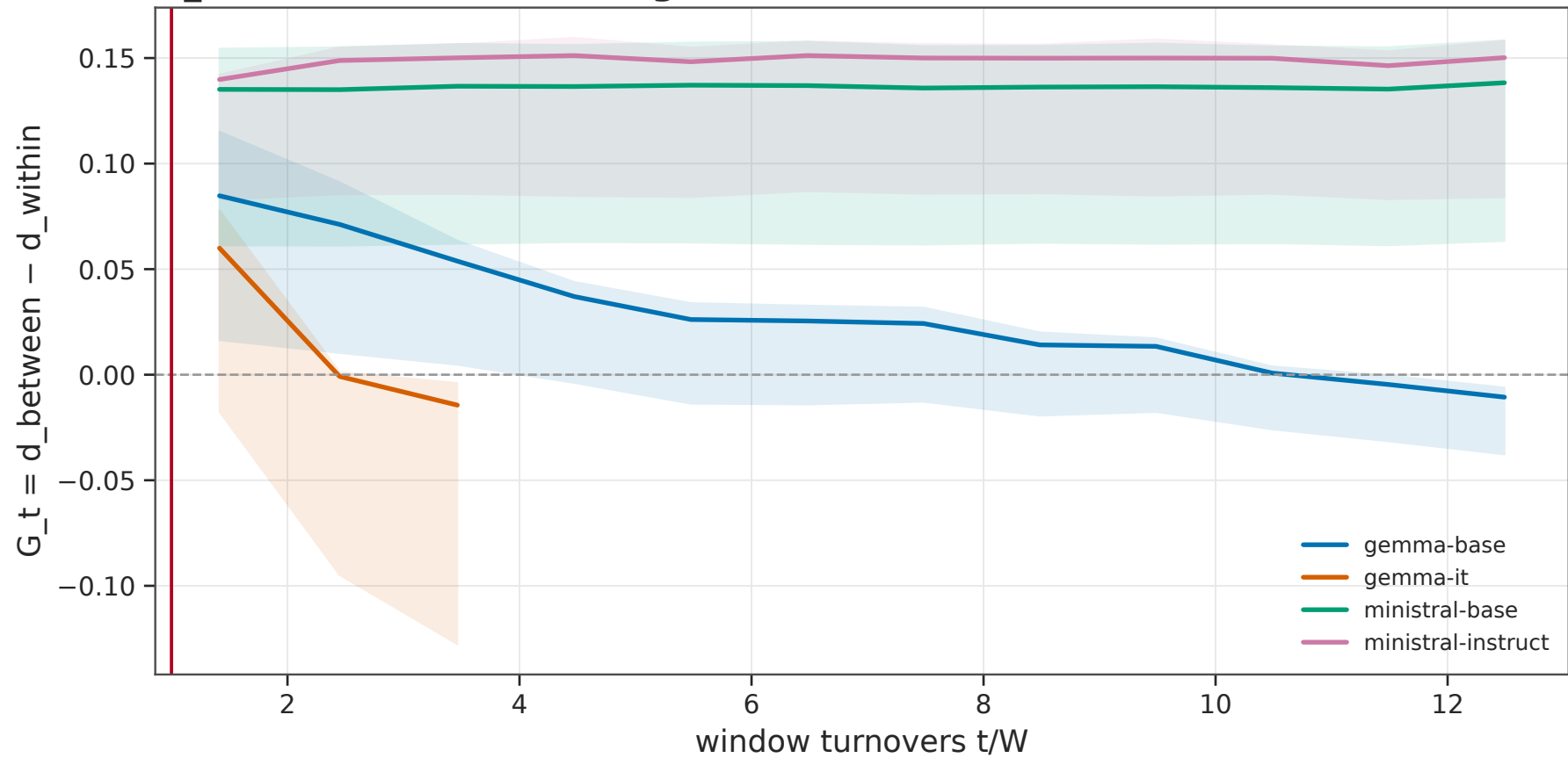
G t vs turnover — local-bge-m3
