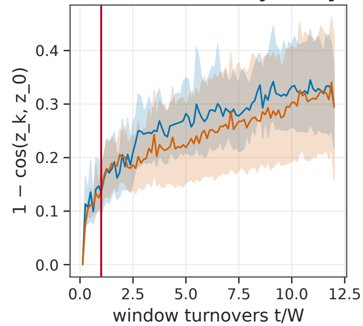
(b) drift from trajectory origin
