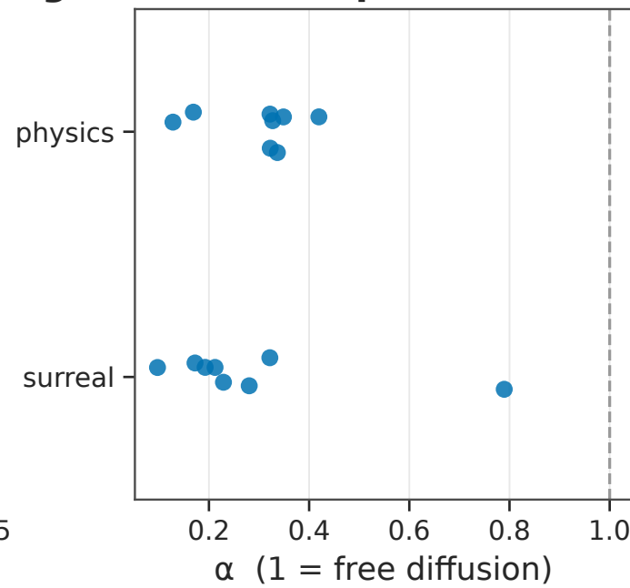
(c) MSD exponent \alpha
