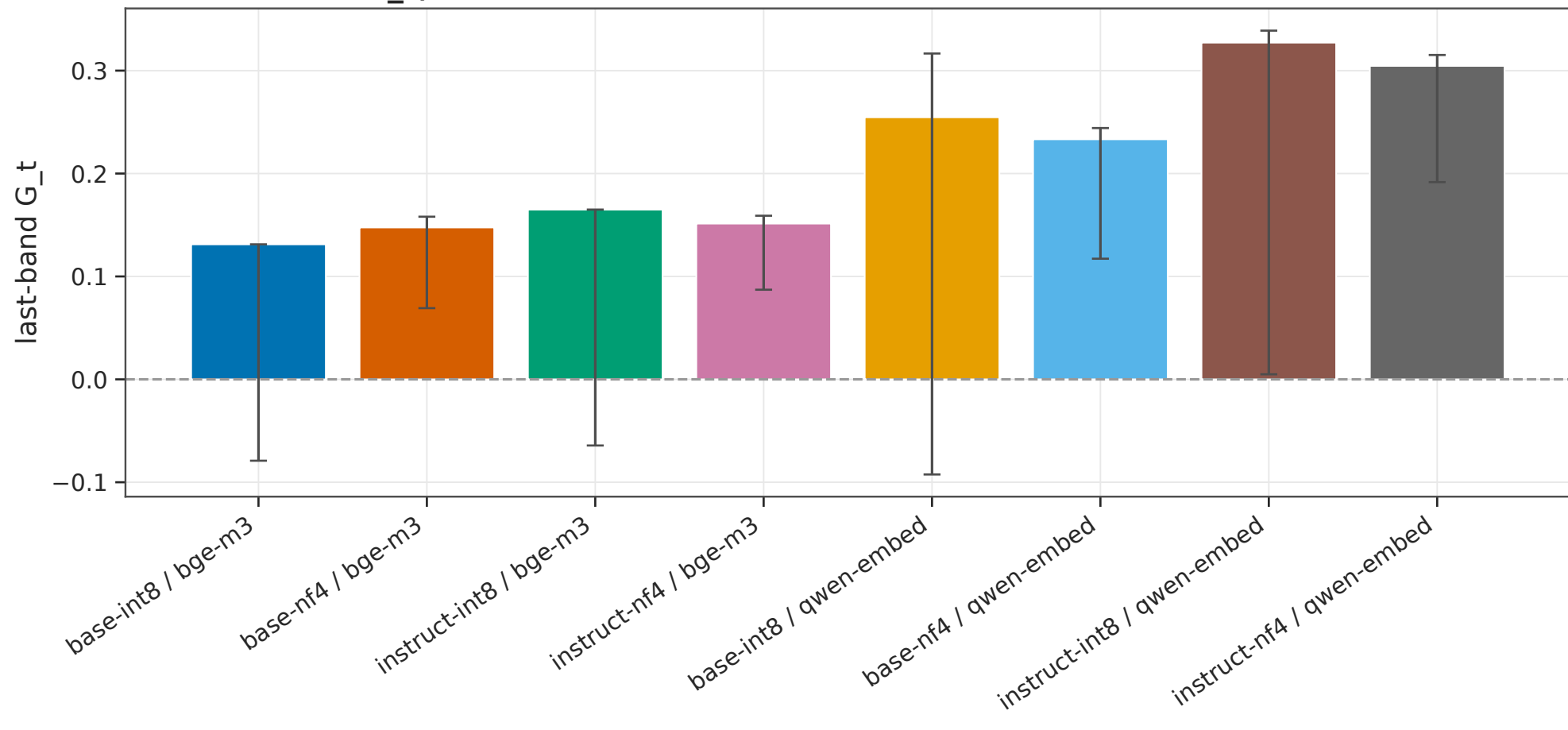
S9 last-band G t , seed-cluster 95% CI
