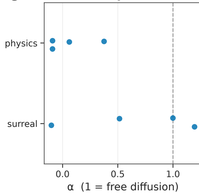
(c) MSD exponent \alpha
