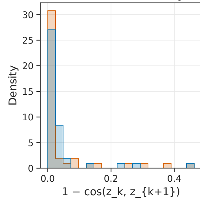
(a) semantic velocity
