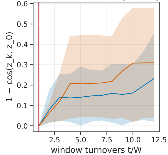
(b) drift from trajectory origin
