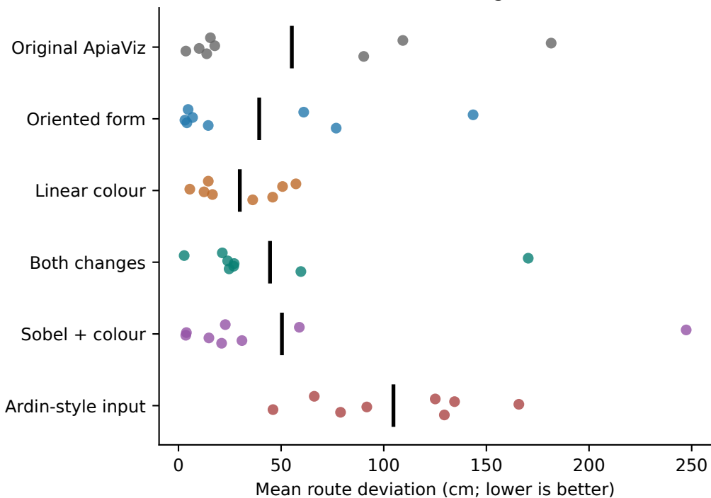
A Each dot is one route, averaged over five seeds
