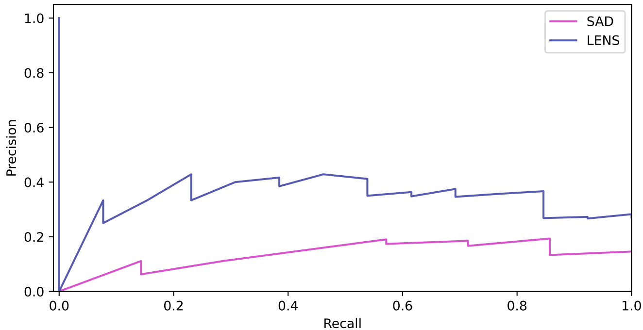
Precision-Recall Comparison
