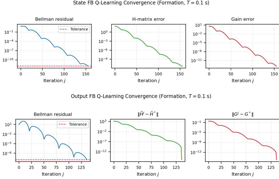
Figure 7: Q-learning convergence for Example 2 ( T = 0.1 s). Top row: state feedback. Bottom row: output feedback.
