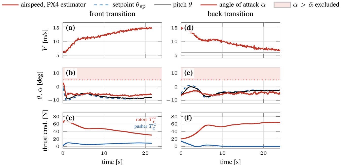
Figure 10: Closed loop with the PX4 firmware in software-in-the-loop, front (left) and back (right) transitions: airspeed from the autopilot's estimator, pitch setpoint sent to the attitude loop with the pitch and angle of attack it produced, rotor and pusher commands.
