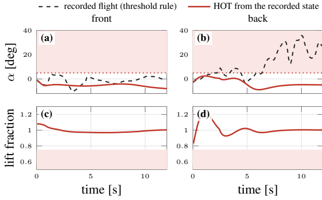
Figure 9: Angle of attack and lift fraction of HOT started from the states recorded in flight (solid) beside the recorded continuation under the threshold rule (dashed), front (left) and back (right).
