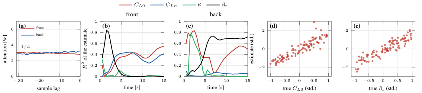
Figure 12: Interpretability on the unseen plants: (a) attention of the context token over the window, front and back, against the uniform weight 1/L ; (b), (c) R^2 of the context-token estimate of the lift-curve offset, the lift-curve slope, the attitude-loop rate and the rotor gain against the true values along the front and the back transition; (d), (e) standardised estimates against the standardised true values at the time of the best R^2 .
