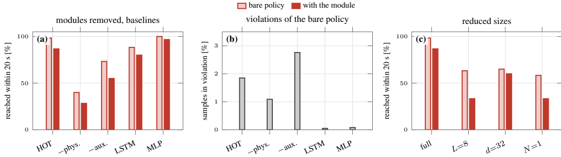
Figure 11: Ablations and parameter analysis on 30 unseen plants, both transitions: (a) fraction of transitions that reach the band within 20 s, bare policy and with the module, for HOT, HOT without the physics features, without the auxiliary head, the LSTM and the MLP; (b) fraction of samples in violation for the bare policies; (c) reach fraction of the reduced sizes (window 8, width 32, one block; trained for 500 iterations).
