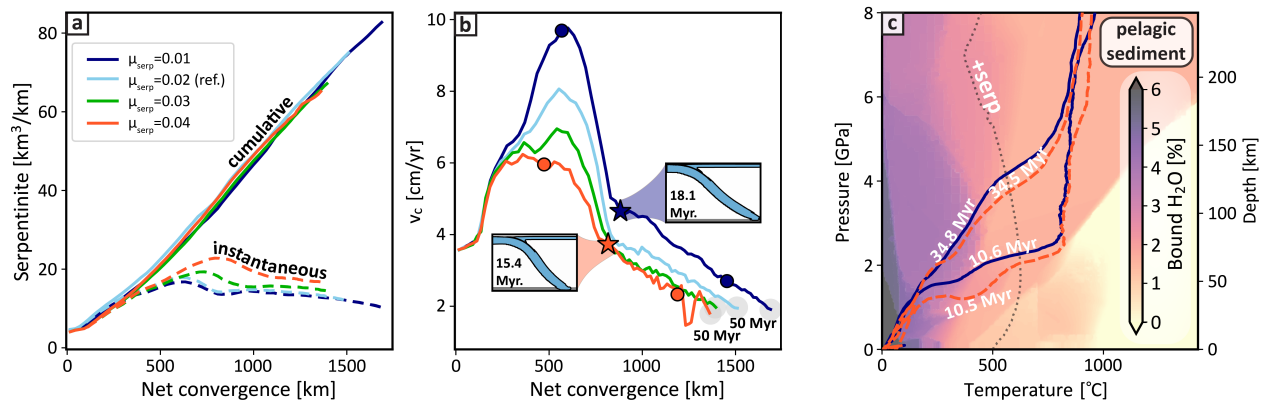
Figure 8. Kinematic and thermal evolution of models with varying the effective friction coefficient of serpentinite. (a) Ingrowth of serpentinite over the course of the model run either considering the cumulative serpentinite amount that was created over the duration of the entire model run or the instantaneous amount that indicates the amount of serpentinite that is stable at any given point in time. The difference between the two is an indication of the degree of loss of serpentinite due to coupling with the downgoing plate. (b) Changes in convergence rate for different models, showing the incorporation of serpentinite into the plate interface. Filled circles denote times when slabtop P-T conditions are plotted in c. (c) The thermal state at two snapshots in time for the strongest and weakest endmembers of serpentinite strength.
