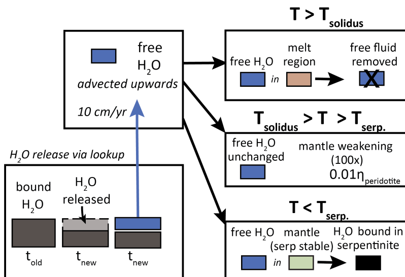
Figure 2. Flowchart illustrating our implementation water release, transport, and storage. Bound H 2 O is calculated with lookups from PerpleX. At each time step new and old H 2 O contents are calculated, and the remaining is
