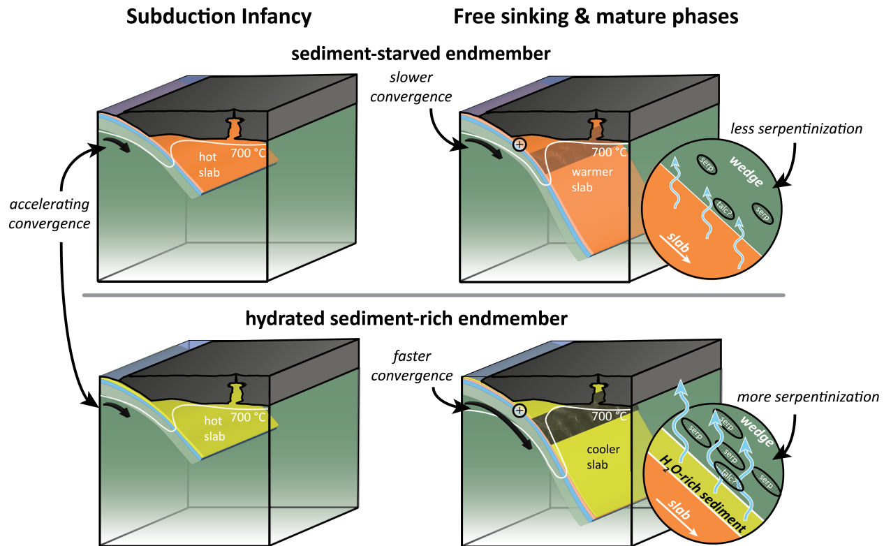
Figure 9. Summary of evolutionary feedback in our numerical results. The ingrowth of serpentinite changes the kinematics, which in turn can change the thermal state over time. All three processes are interconnected and can accentuate the influence of hydrated subducting lithologies, such as sediment, on convergence rates. Shaded regions in free sinking/mature phase correspond to regions of active serpentinization.
