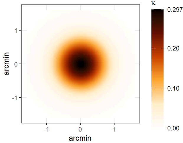
Figure 1: True convergence map \kappa_{\text{true}}(\theta) used throughout the simulation study. The Gaussian cluster profile peaks at \kappa_0 = 0.297 with scale radius \sigma_\ell = 0.5 arcmin. The field is 3.2 \times 3.2 arcmin \{\}^2 on a 32 \times 32 pixel grid.
