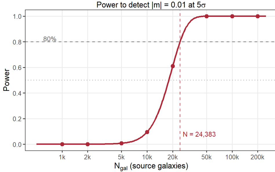
Figure 3: Power to detect |m| = 0.01 at 5-sigma significance as a function of the number of source galaxies N_{\text{gal}} , for B = 500 replicates per condition. The dashed crimson line marks the 80% power threshold at N_{\text{gal}} \approx 24,383 .
