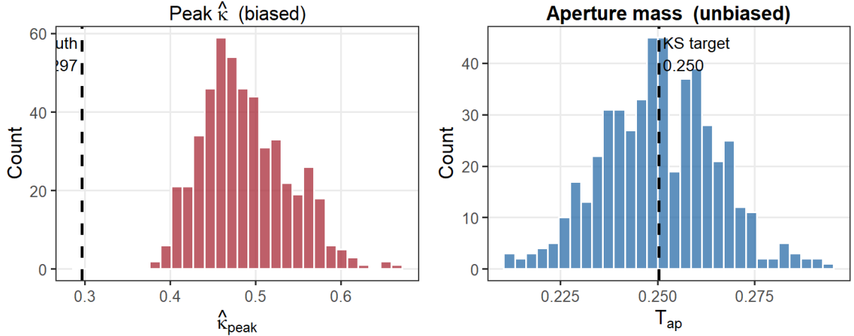
Figure 2: Monte Carlo distributions of peak \hat{\kappa} (left) and aperture mass T_{\text{ap}} (right) across B = 500 replicates. The dashed vertical line marks the target value in each case. Peak \hat{\kappa} is severely upward-biased by noise spikes; aperture mass is nearly unbiased relative to the noiseless KS target.
