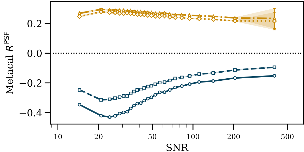
Metacalibration R^{\text{PSF}}
