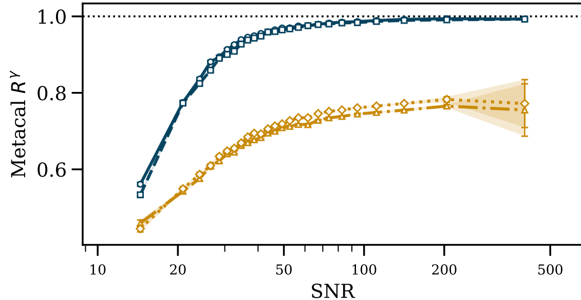
Metacalibration R^Y
