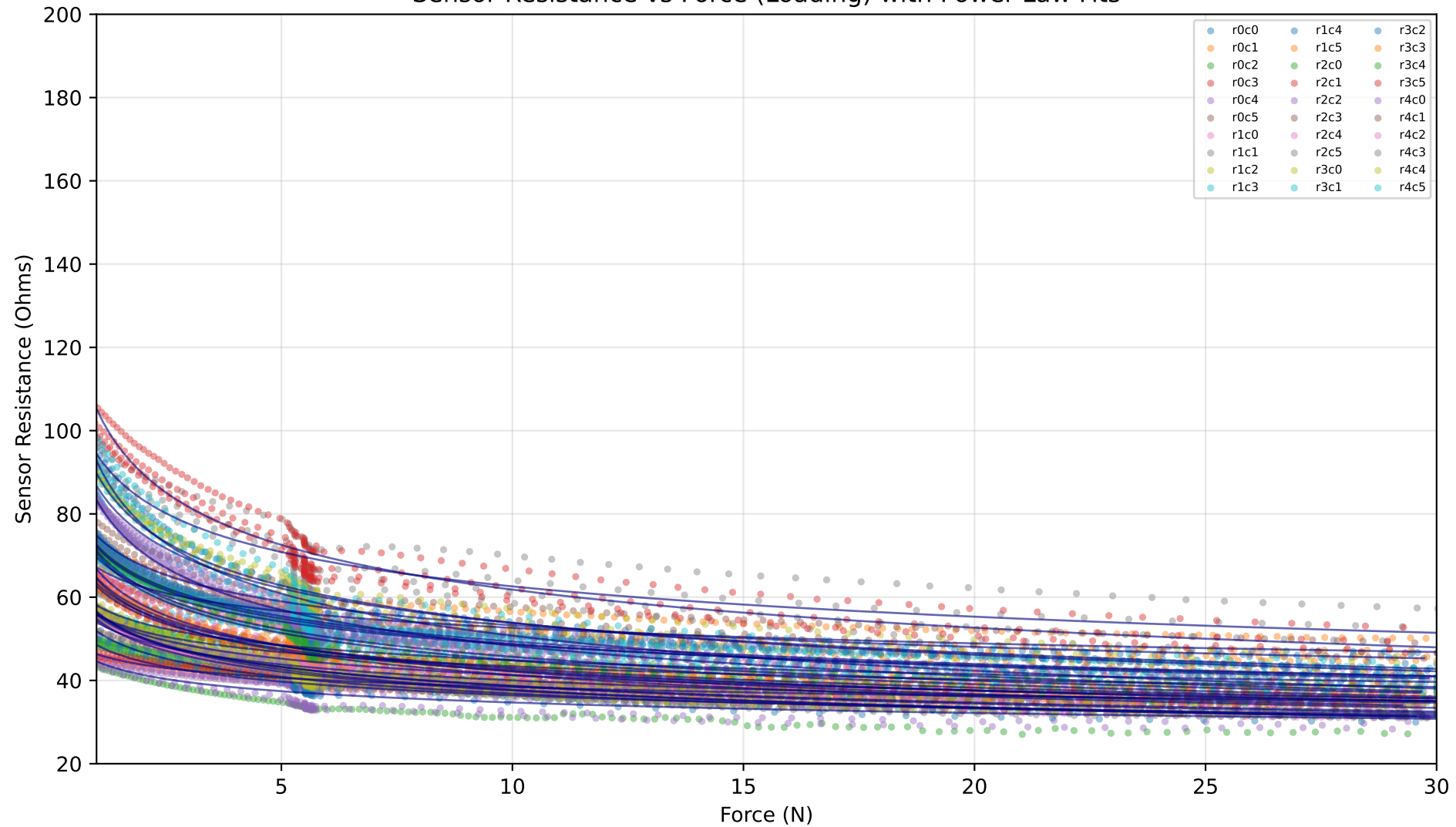
Sensor Resistance vs Force (Loading) with Power-Law Fits
