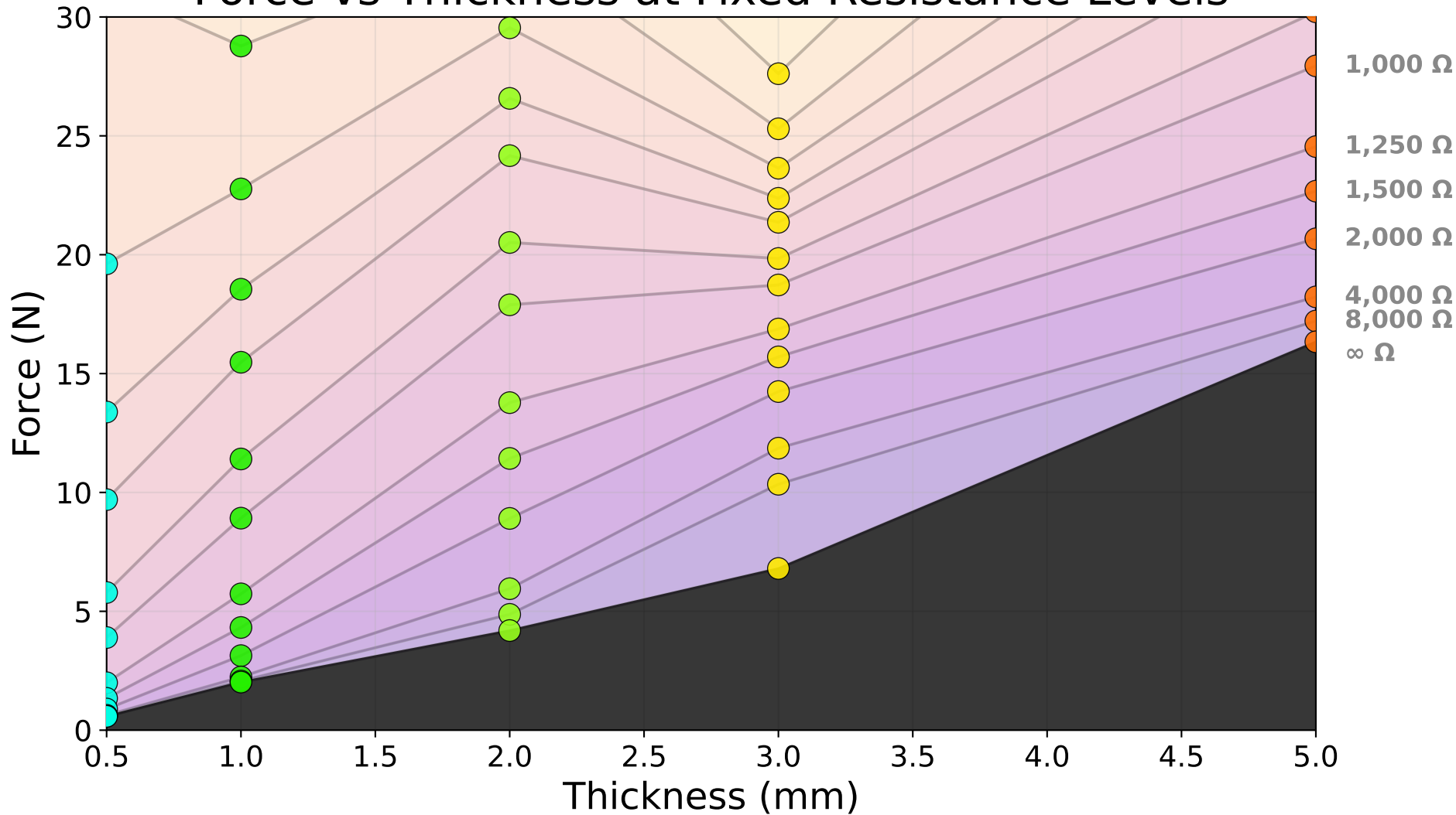
Force vs Thickness at Fixed Resistance Levels
