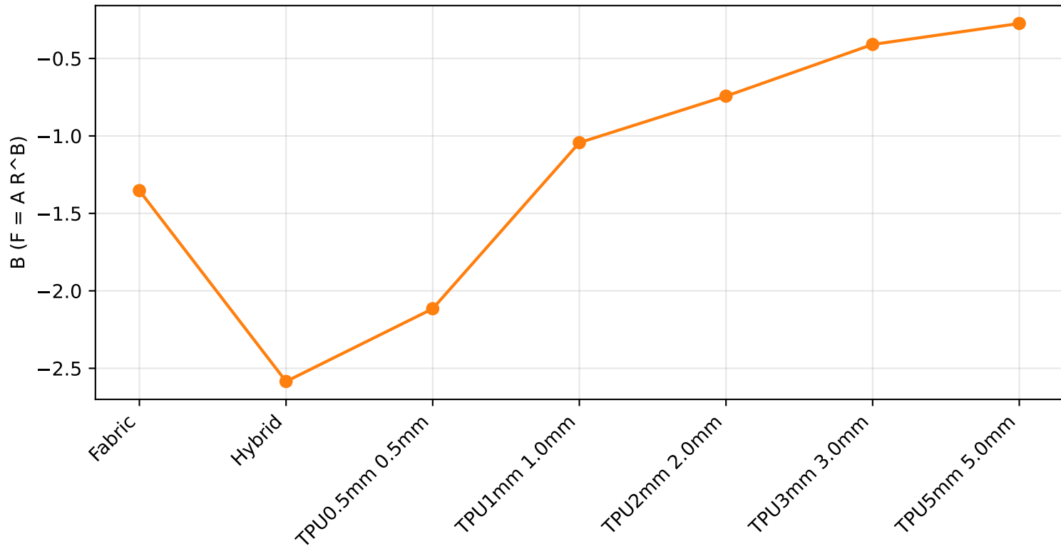
Power-law B by Type
