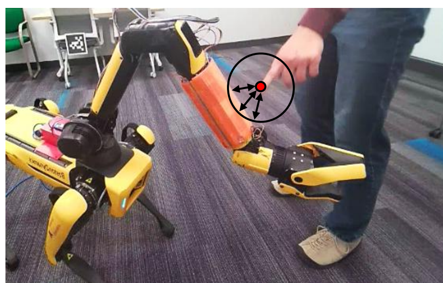
ContactIK
