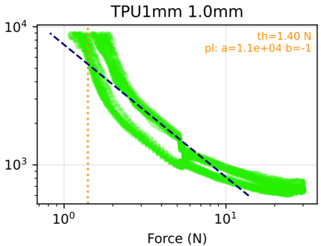
Log-Log: Force vs Sensor Resistance by Type (Loading)
