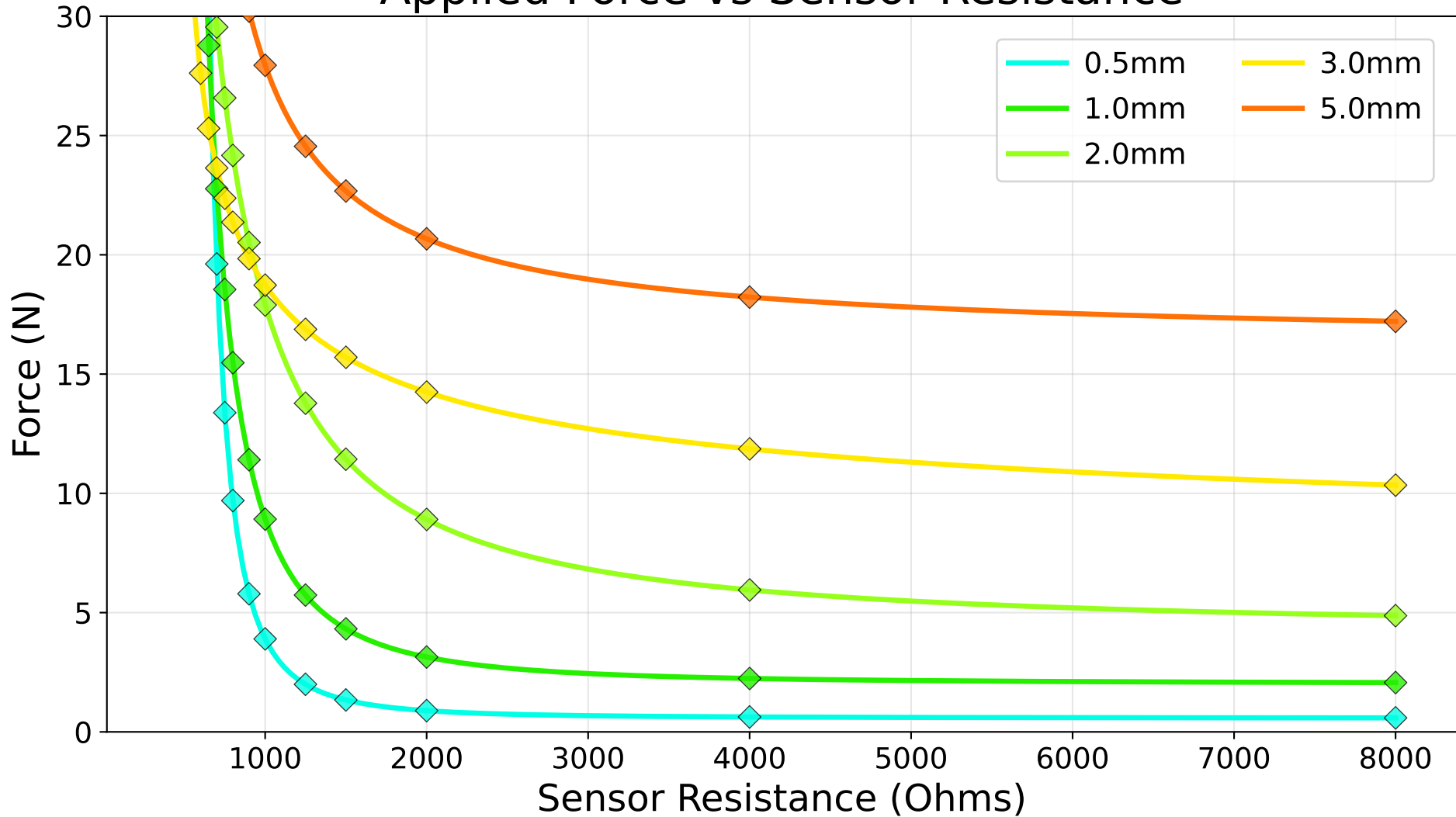
Applied Force vs Sensor Resistance
