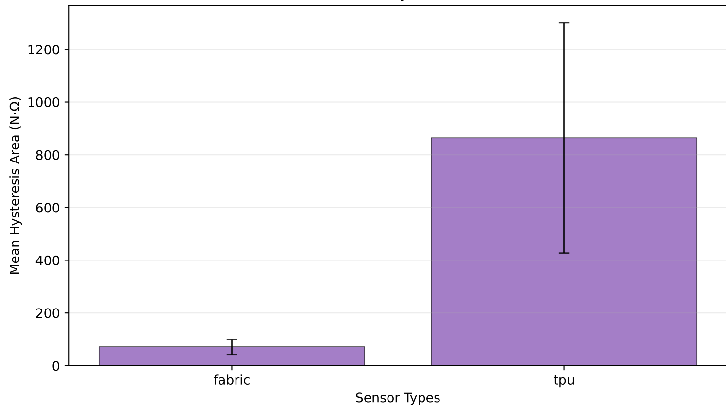
Overall Hysteresis
