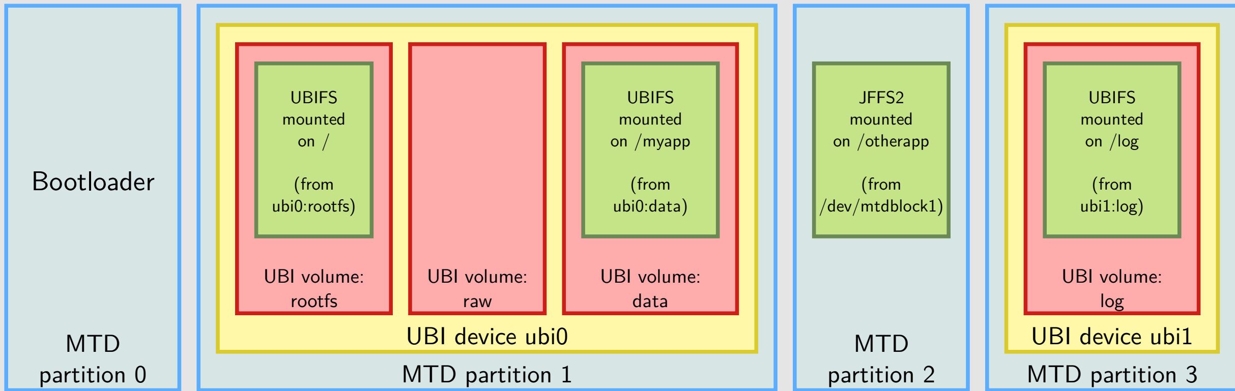
Flash device layout: bad example
