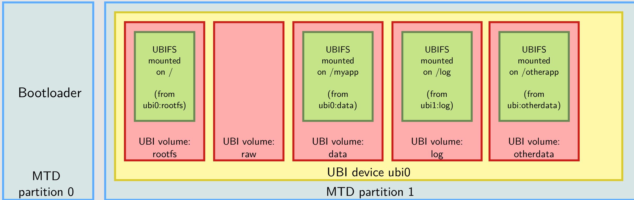
Flash device layout: good example
