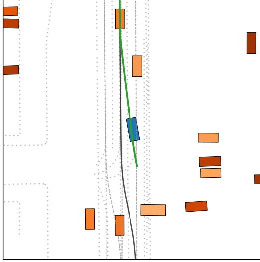
Figure 7: Example render of Waymax.
