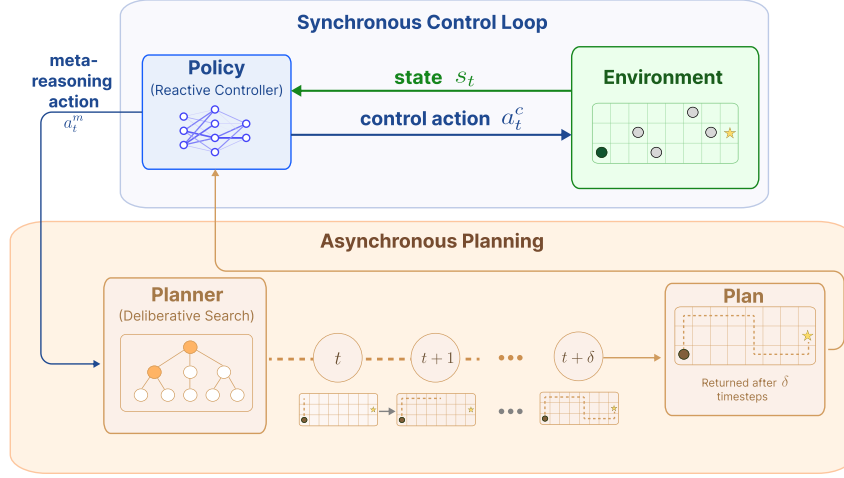
Figure 1: Visualization of the real-time meta-reasoning MDP. In this MDP we formally analyze when policy improvement selects a plan action instead of a control action and propose an RL-based method AWT to train agents to operate in real-time domains with slow, asynchronous planners.
