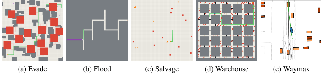
Figure 2: Visual representation of our suite of environments. In all environments the agent is blue and the plan is green . In all gridworlds, and the goal(s) are orange . In Evade, Salvage, and Warehouse, objects which move around the world in a predefined motion are red . In Evade and Flood, objects which pursue the agent are purple . In Waymax, the desired path is in black .
