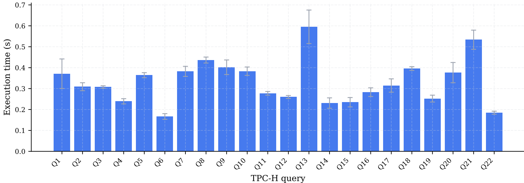
TPC-H Query Execution Times — Docker, SF1 (3 measured runs, 1 warmup)
