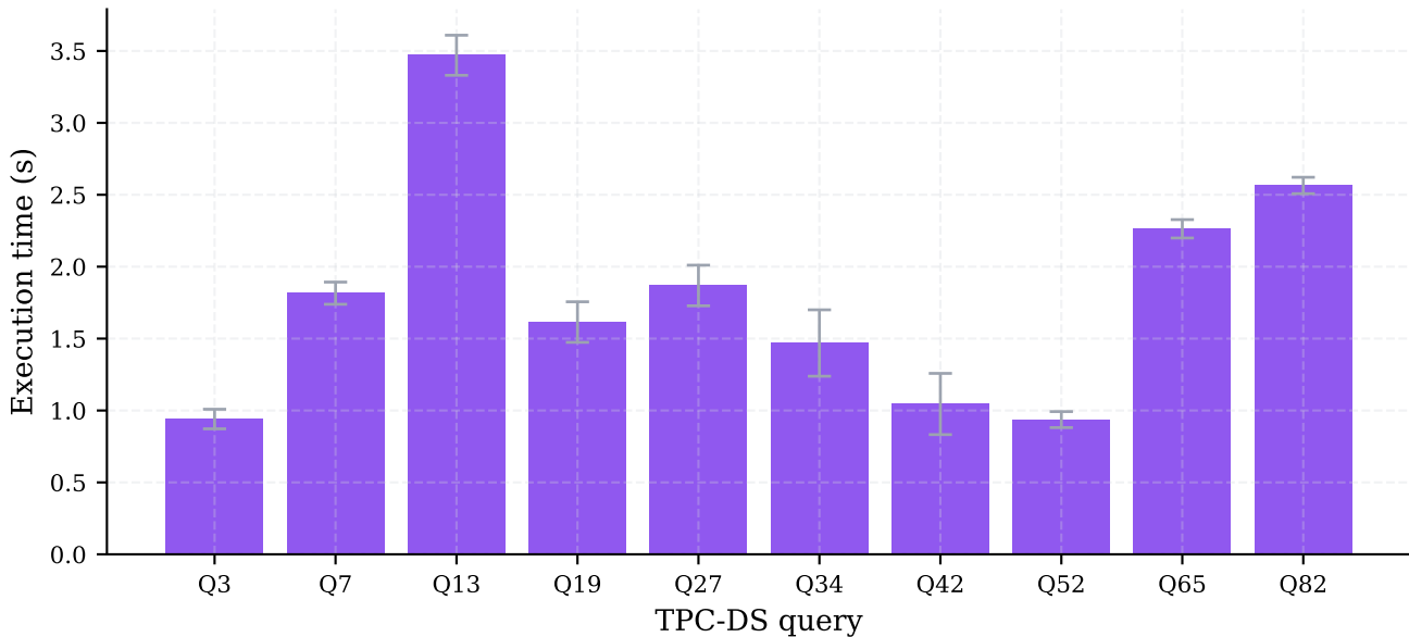
TPC-DS Query Latencies — GPG Bare-Metal K8s, SF10, 2 workers (5 runs)
