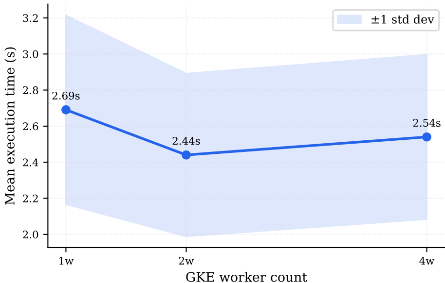
Mean TPC-H Query Latency vs Worker Count — GKE, SF1
