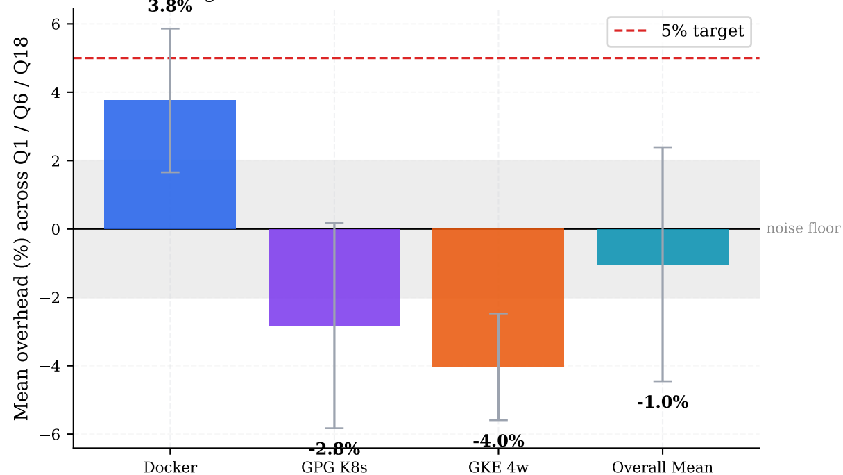
Mean Monitoring Overhead — TriBench instrumented vs uninstrumented
