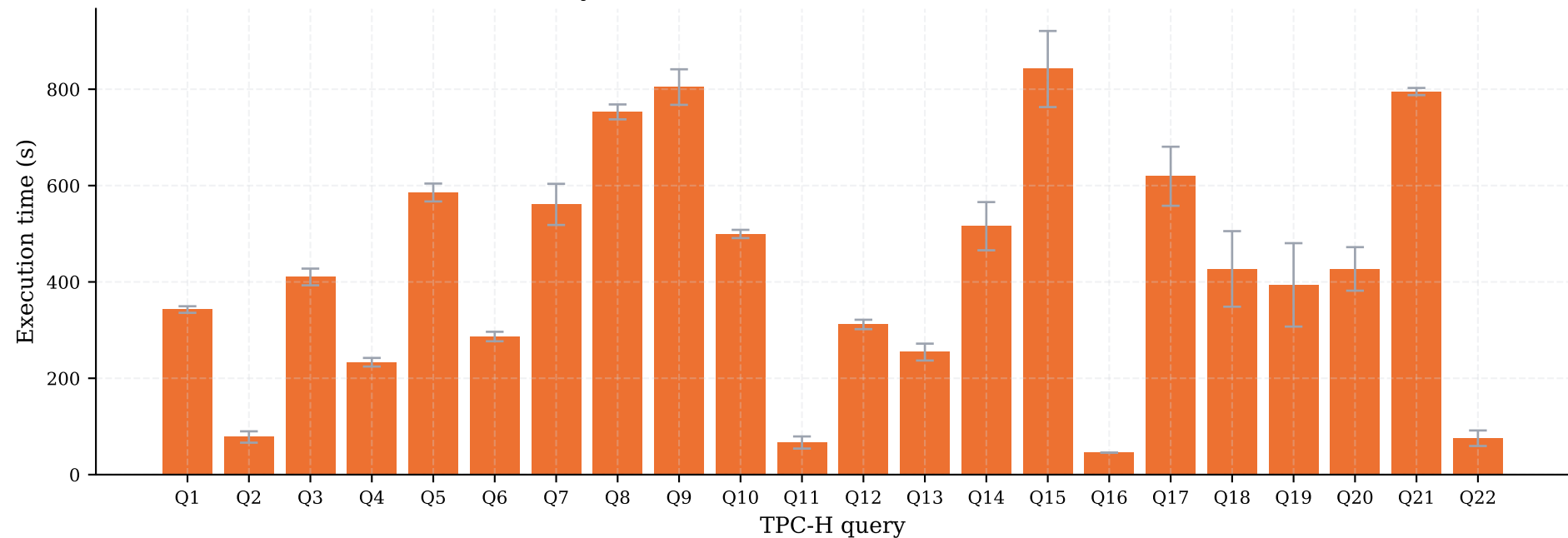
TPC-H Query Latencies — GKE 4-Worker Cluster, SF100 (3 runs)
