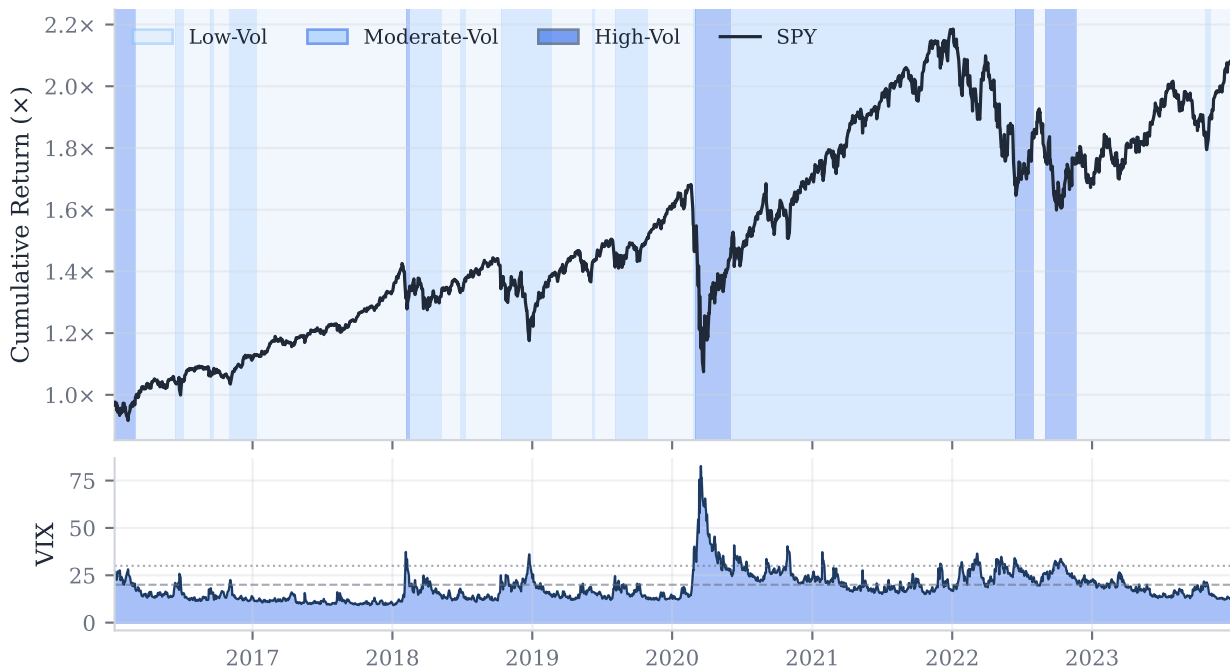
HDP-HMM Regime Timeline (January 2016–December 2023)
