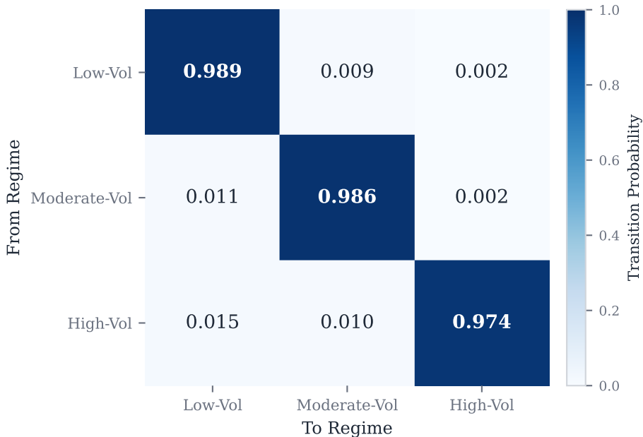
HDP-HMM Posterior-Mean Transition Matrix
