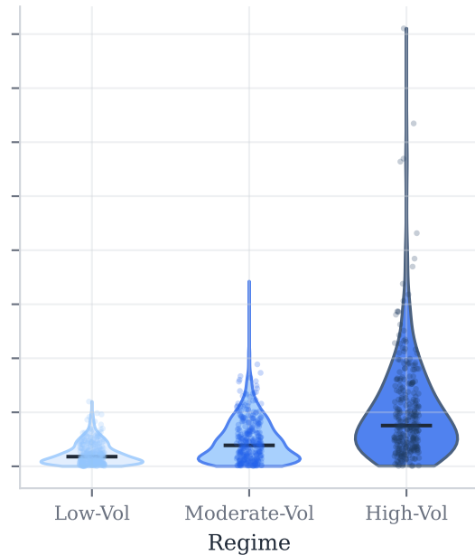
VIX Threshold
