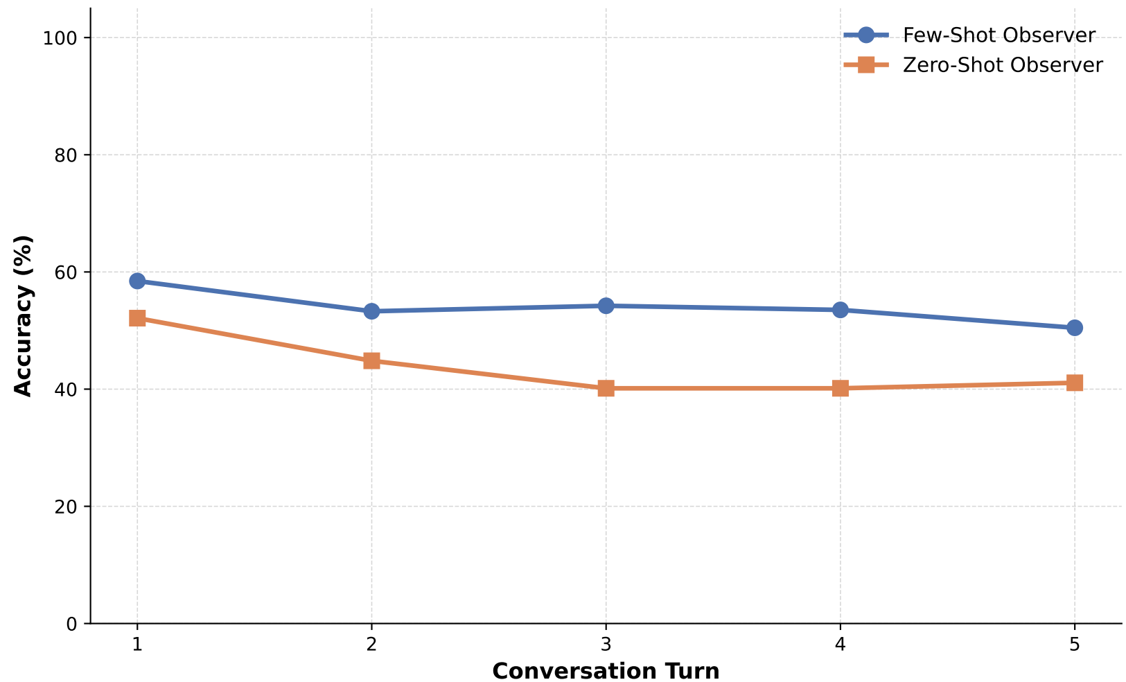
LLM Observer Accuracy by Conversation Turn (Neutral Dataset)
