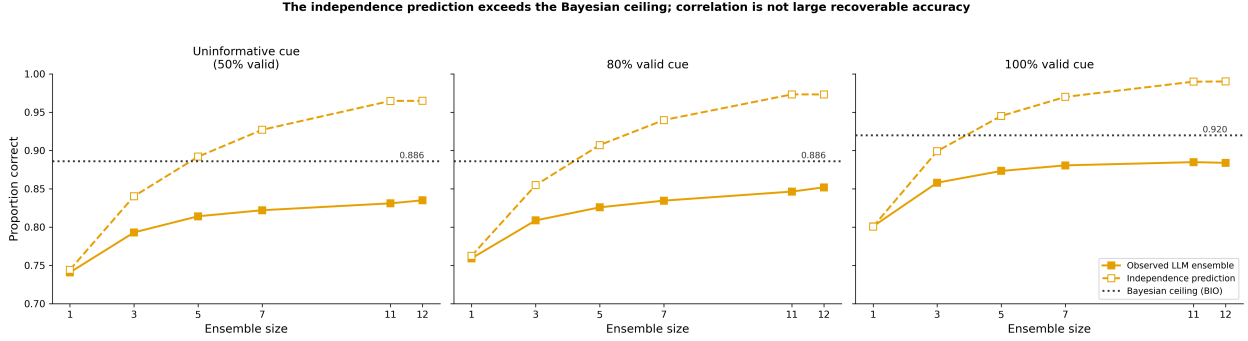
Figure 3: Observed LLM ensemble accuracy (solid) against two reference lines, by group size and condition. The independence prediction (dashed) is the Condorcet majority-vote accuracy the same agents would reach if their errors were fully independent, computed by permuting each agent’s per-trial correctness. The Bayesian ideal observer ceiling (dotted) is the highest accuracy any decision-maker can reach with this stimulus information. The independence prediction sits above the ideal observer, which is not achievable: it removes correlation that is structural to the task, since a genuinely ambiguous stimulus misleads every agent at once. The meaningful comparison is observed against the ideal observer, a gap of only a few points for the LLM ensemble. Correlation is why the gains stop early, not a large amount of recoverable accuracy.
